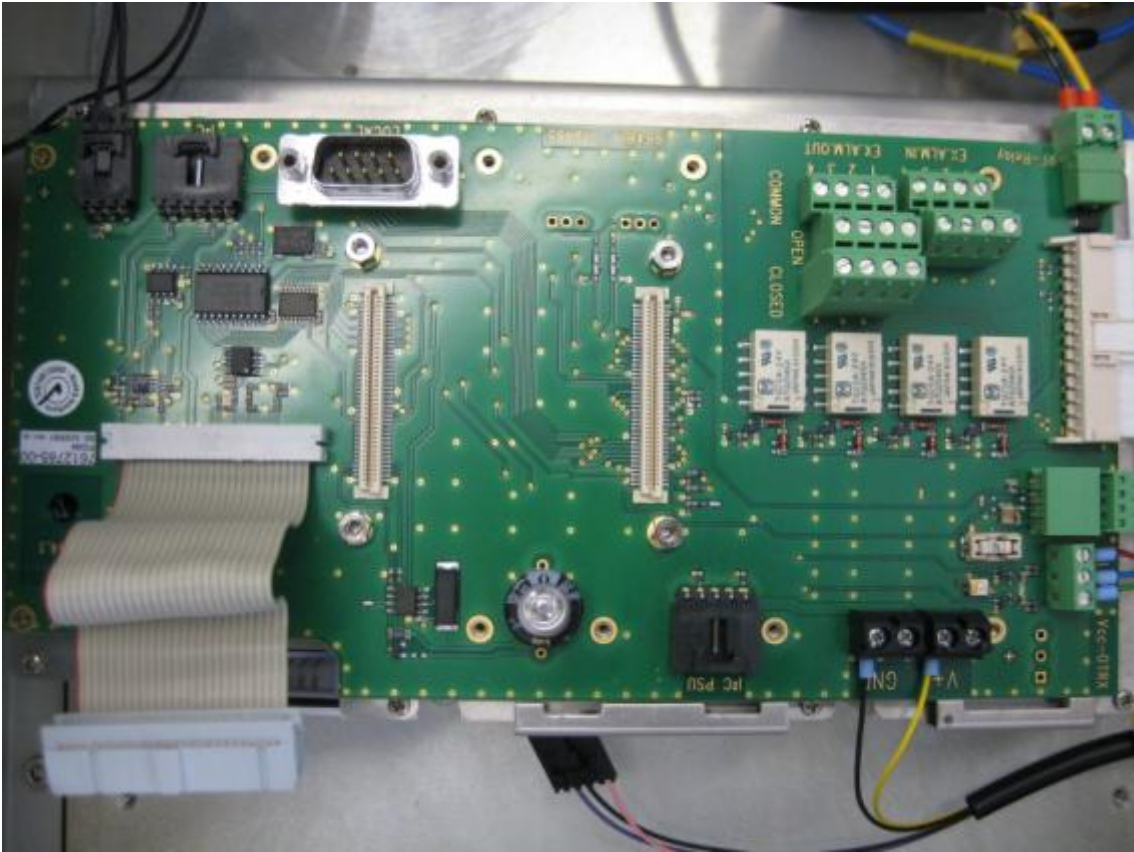
Controlboard Top
