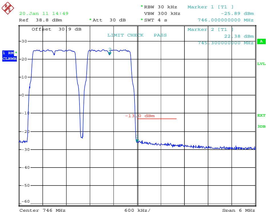
plot 7.3.1.1-#2 Spurious Emissions at Antenna Terminals: §27.53, §2.1051; RSS-131, RSS-GEN; Test results; Downlink; LTE < 1MHz to band edge 728 – 746MHz, MIMO Upper Band Edge
