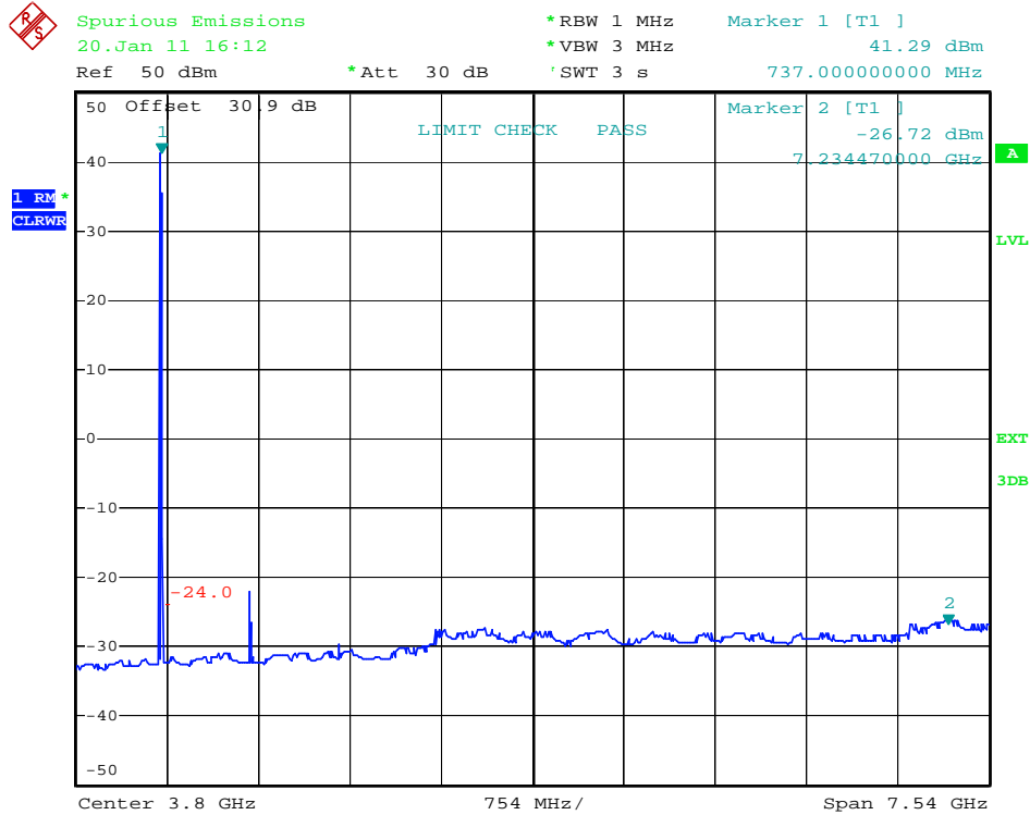
plot 7.3.1.3-#1 Spurious Emissions at Antenna Terminals: §27.53, §2.1051; RSS-131, RSS-GEN; Test results; Downlink; LTE > 1MHz to band edge 728 – 746MHz, MIMO;
