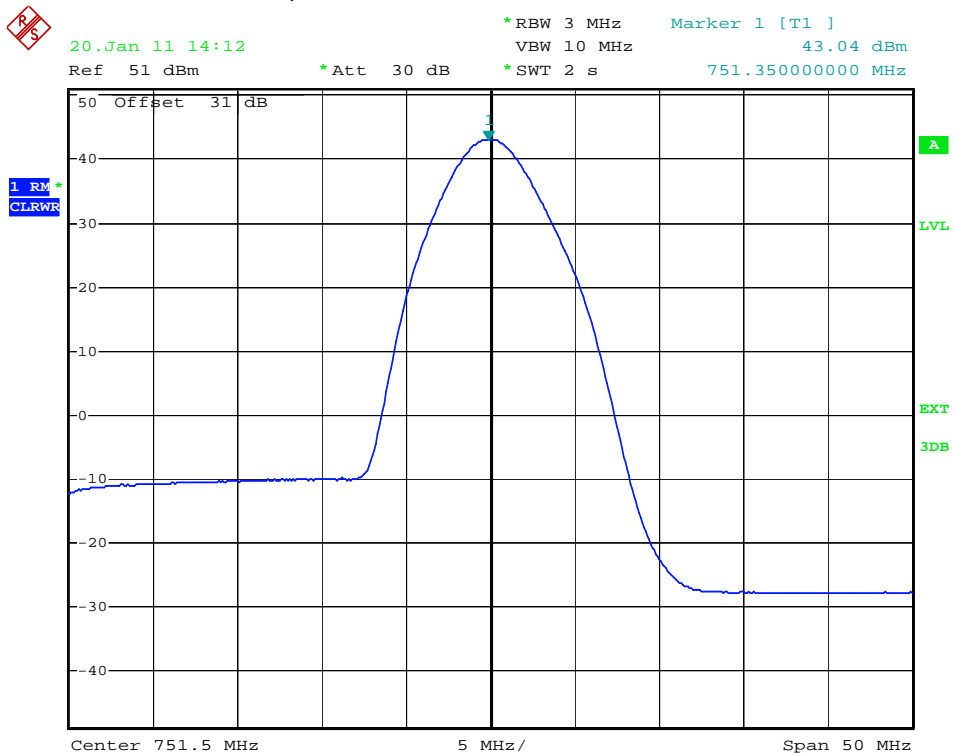
plot 5.3.1.2-#2 RF Power Out: §27.50, §2.1046; RSS-131, RSS-GEN; Test Results; Downlink; LTE 746 – 757MHz, MIMO Middle
