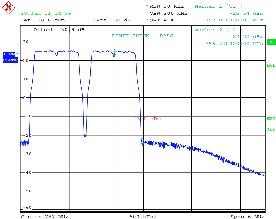
plot 7.3.1.2-#2 Spurious Emissions at Antenna Terminals: §27.53, §2.1051; RSS-131, RSS-GEN; Test results; Downlink; LTE < 1MHz to band edge 746 – 757MHz, MIMO Upper Band Edge
