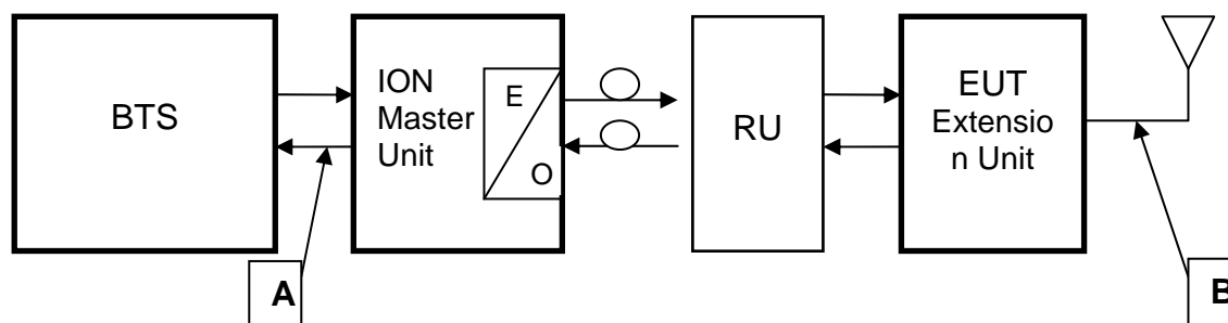
figure 2.1.5-#1 Block diagram of measurement reference points
