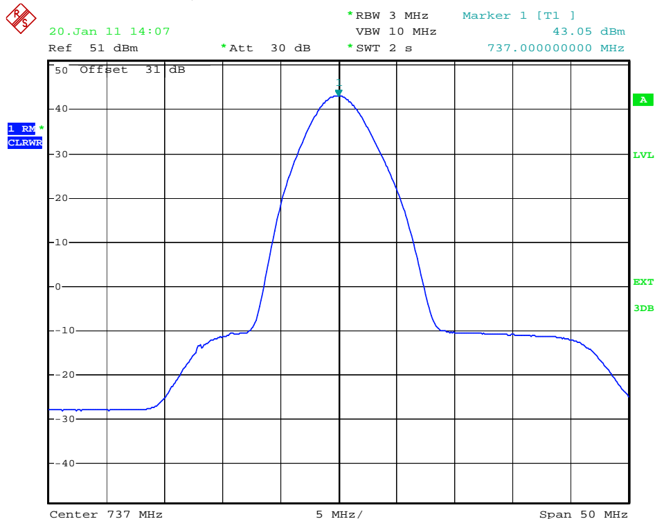
plot 5.3.1.1-#2 RF Power Out: §27.50, §2.1046; RSS-131, RSS-GEN; Test Results; Downlink; LTE 728 – 746MHz, MIMO Middle
