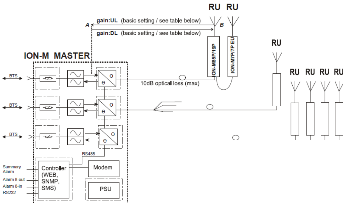
figure 2.1.4-#1 System diagram of EUT: ION-M7P/7P_EU
