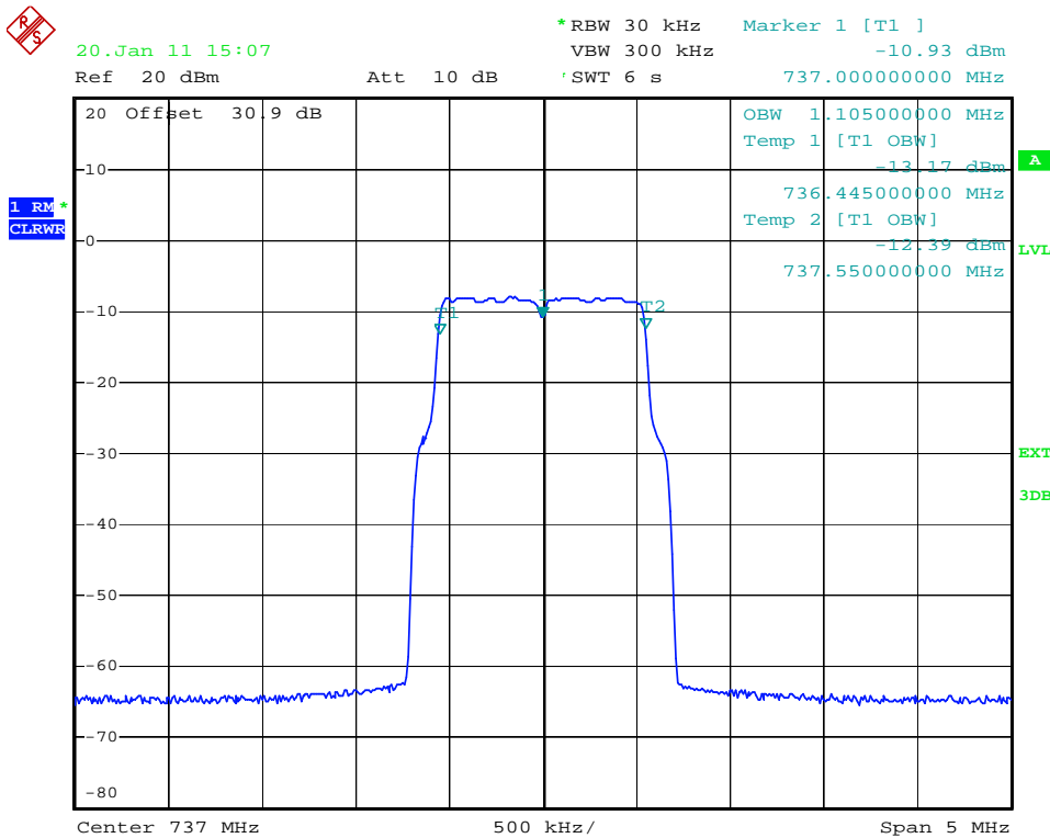
plot 6.3.1.1-#2 Occupied Bandwidth: §90.210, §2.1049; RSS-GEN; Test results; Downlink; LTE 728 – 746MHz MIMO Input
