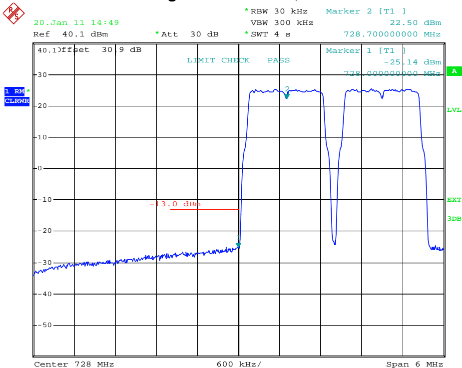
plot 7.3.1.1-#1 Spurious Emissions at Antenna Terminals: §27.53, §2.1051; RSS-131, RSS-GEN; Test results; Downlink; LTE < 1MHz to band edge 728 – 746MHz, MIMO Lower Band Edge
