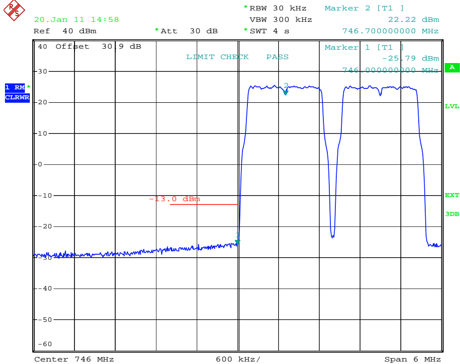
plot 7.3.1.2-#1 Spurious Emissions at Antenna Terminals: §27.53, §2.1051; RSS-131, RSS-GEN; Test results; Downlink; LTE < 1MHz to band edge 746 – 757MHz, MIMO Lower Band Edge
