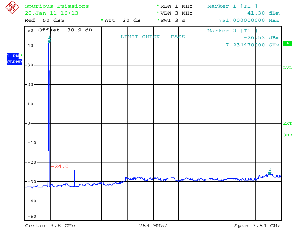
plot 7.3.1.4-#1 Spurious Emissions at Antenna Terminals: §27.53, §2.1051; RSS-131, RSS-GEN; Test results; Downlink; LTE > 1MHz to band edge 746 – 757MHz, MIMO;
