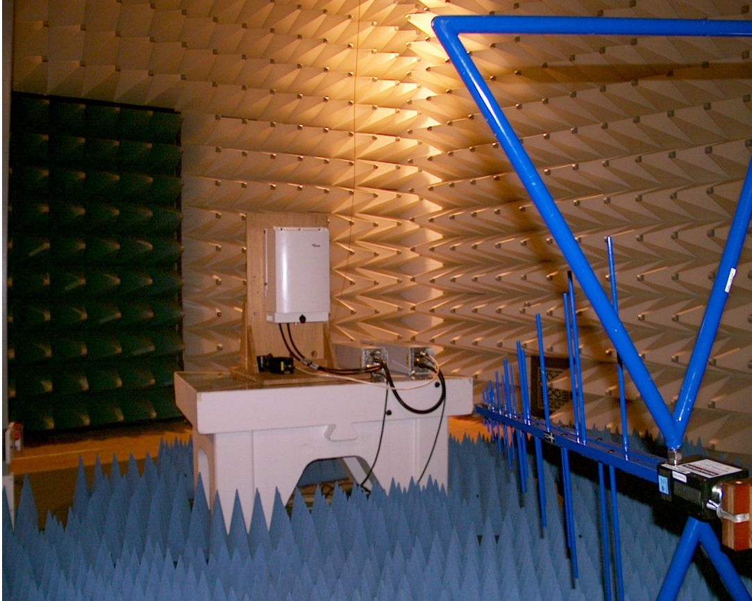
RE<1GHz @3m FAC
