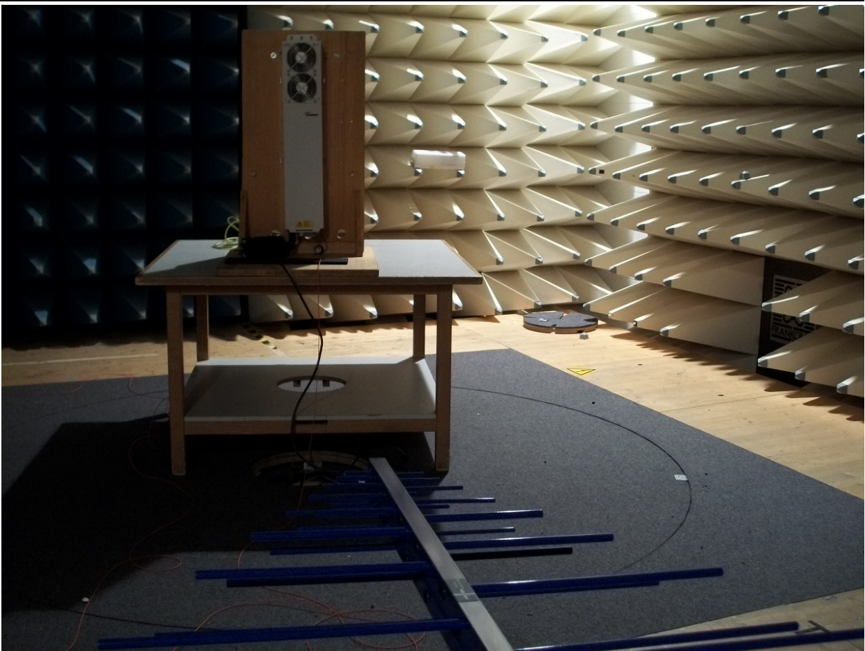
picture 8.2: Test setup: Field Strength Emission < 1 \text{ GHz} @3m in the FAC
