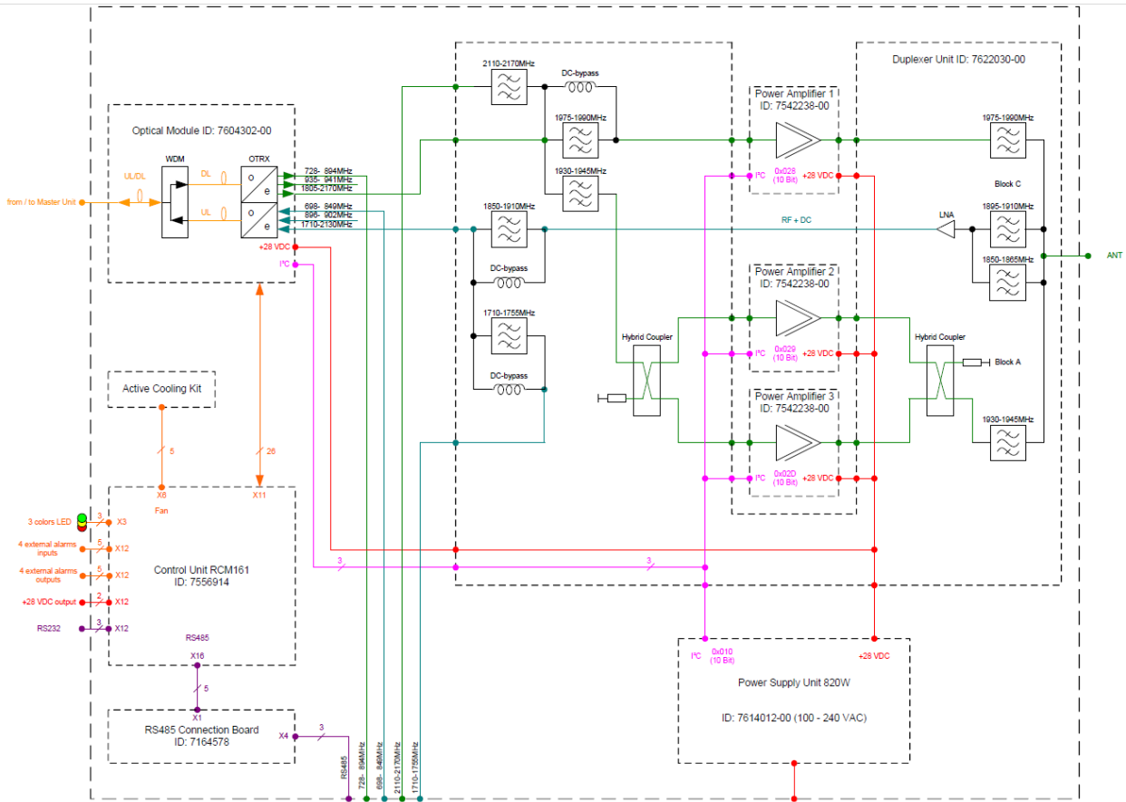
figure 2.1.4-#1 System diagram of EUT: ION optical distribution system
