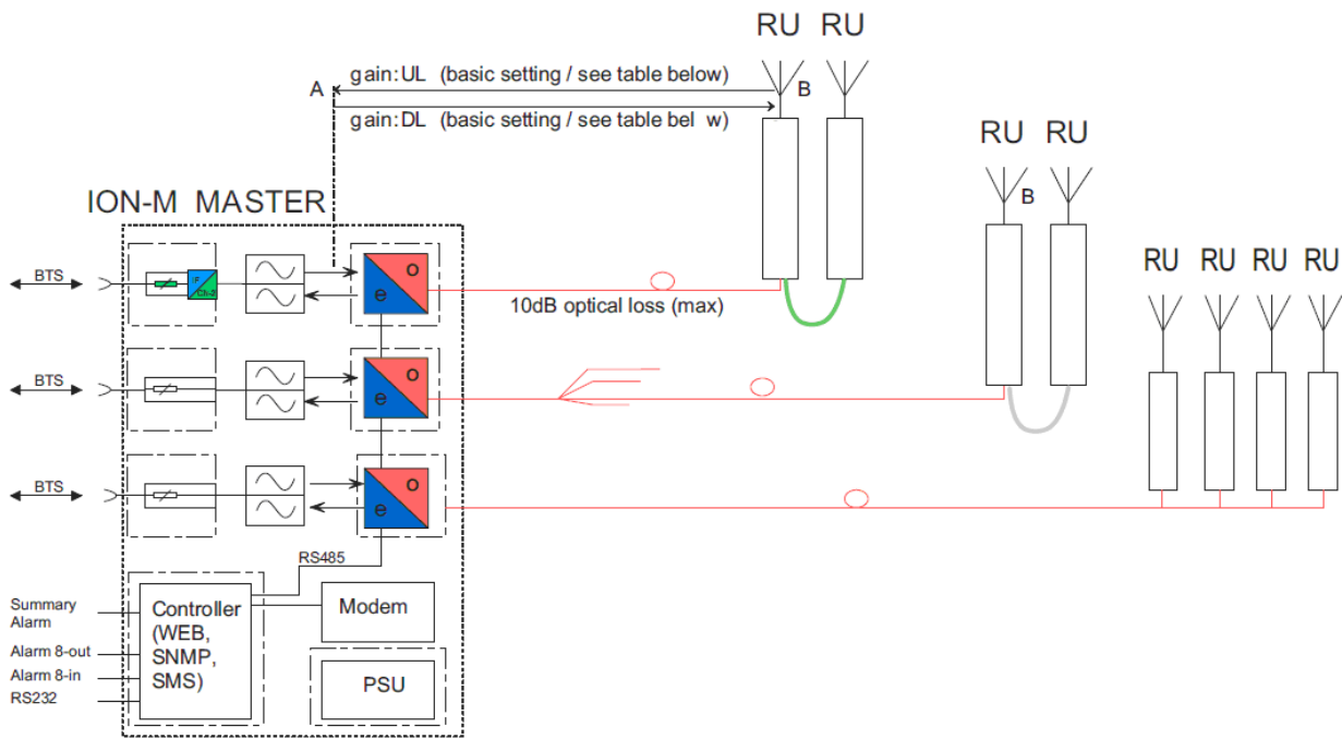
figure 2.1.4-#2 System diagram of EUT: EUT is Remote Unit
