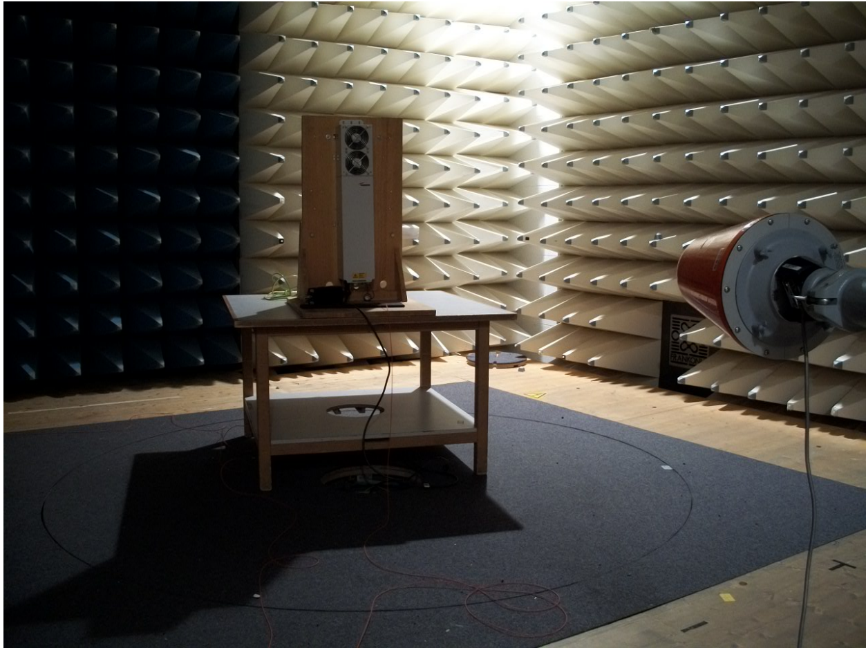
picture 8.1: Test setup: Field Strength Emission 1GHz to 22GHz @3m in the FAC
