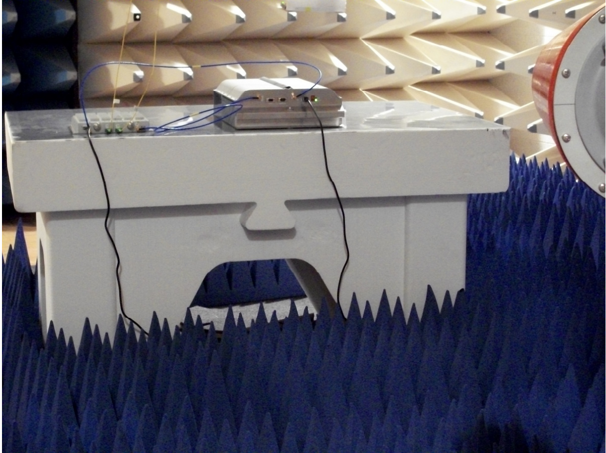
Radiated Spurious Emission >1GHz
