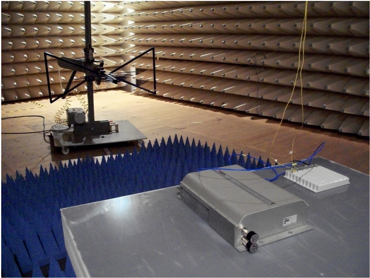
Radiated Spurious Emissions <1GHz
