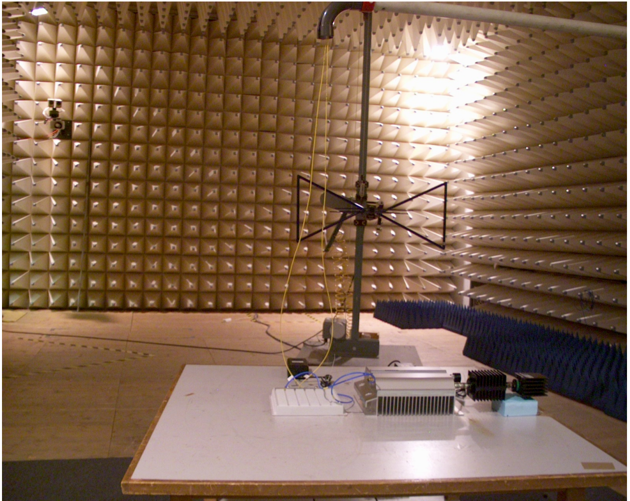
picture 2: Test setup: Field Strength Emission <math>< 1\text{ GHz}</math> @3m in the FAC
