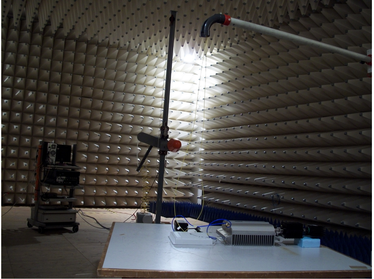
picture 1: Test setup: Field Strength Emission >1 GHz @3m in the FAC
