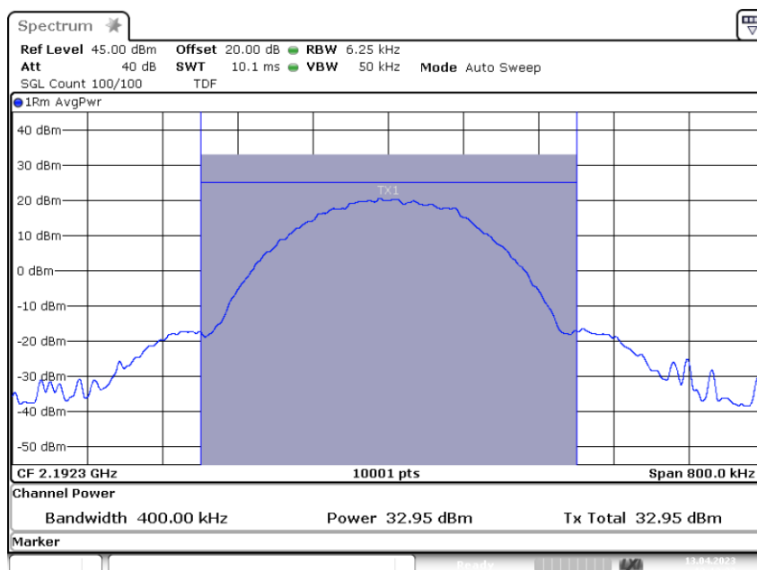
3.5.3 Power GSM Out +3 2.19230G
