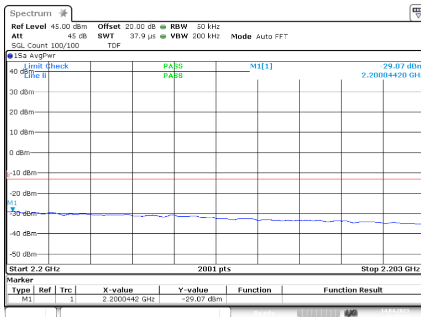
3.6.2 out of band emi AWS1700E_high AWGN upper lcarrier -0.3 dB 2.200G 2.203G
