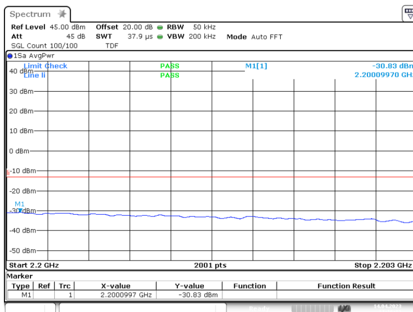
3.6.2 out of band emi AWS1700E_high AWGN upper lcarrier +3.0 dB 2.200G 2.203G
