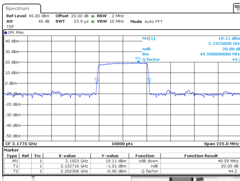
3.3 Out of band rejection AWS1700E_high 2.17750G _20dB
