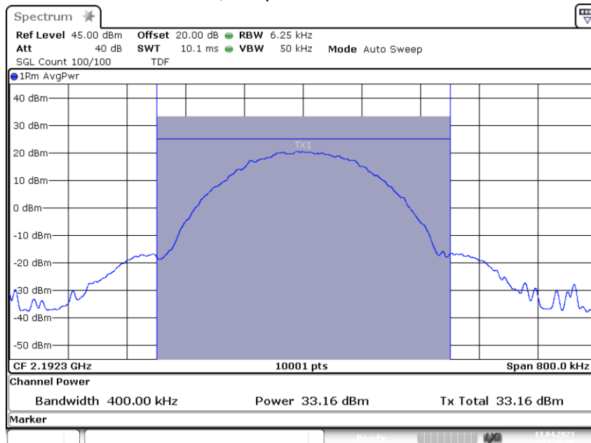
3.5.3 Power GSM Out -0.3 2.19230G
