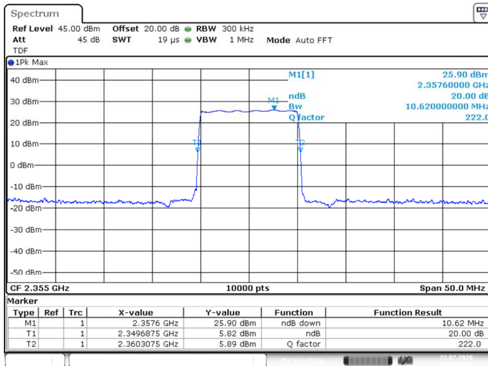
3.3 Out of band rejection WCS2300 2.35500G _20dB
