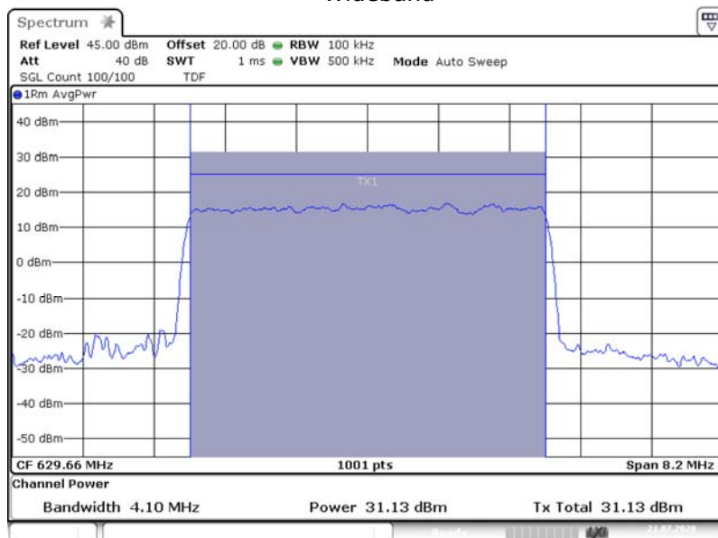
3.5.3 Power AWGN Out +3 629.66000M
