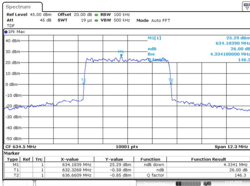
Output Signal
