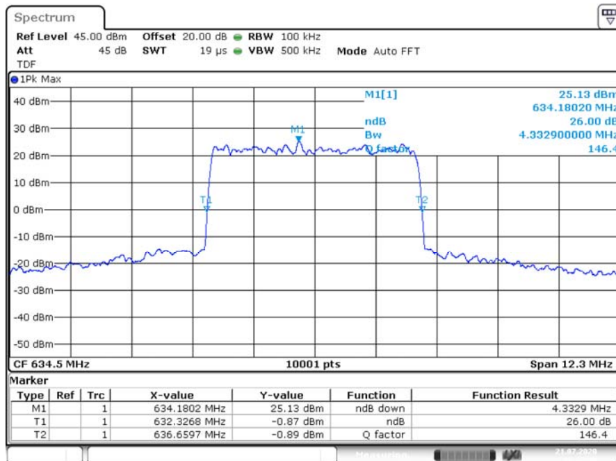
Output Signal
