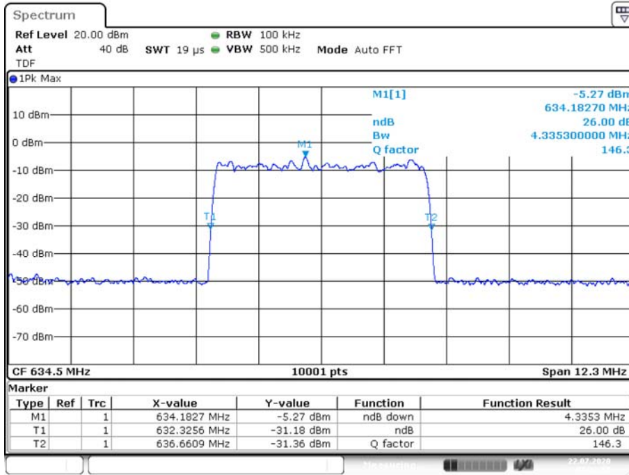
Input Signal
