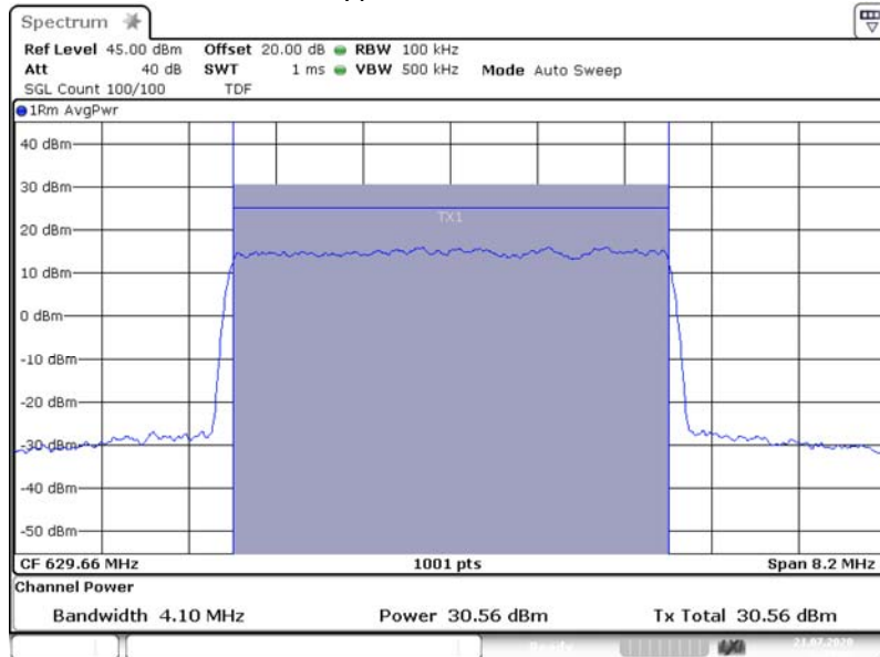
3.5.3 Power AWGN Out -0.3 629.66000M
