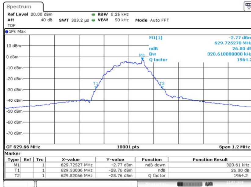
Input Signal
