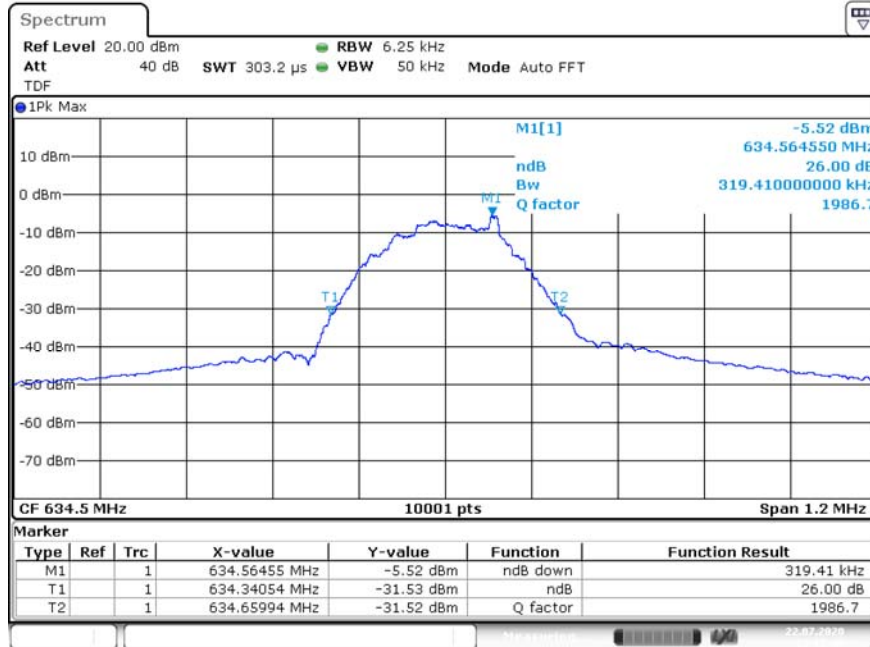
Input Signal
