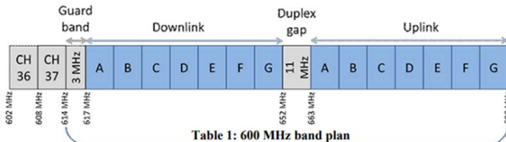
Figure 1: 600 MHz Band Plan
