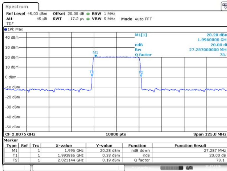
3.3 Out of band rejection Band70 2.00750G _20dB
