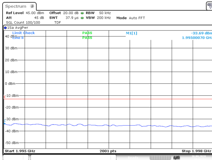
3.6.2 out of band emi PCS1900 AWGN upper 1carrier -0.3 dB 1. 995G 1.998G
