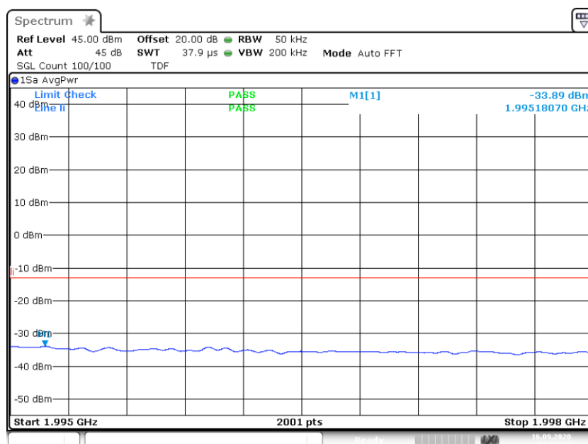
3.6.2 out of band emi PCS1900 AWGN upper 1carrier +3.0 dB 1. 995G 1.998G
