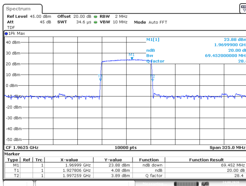
3.3 Out of band rejection PCS1900 1.96250G _20dB
