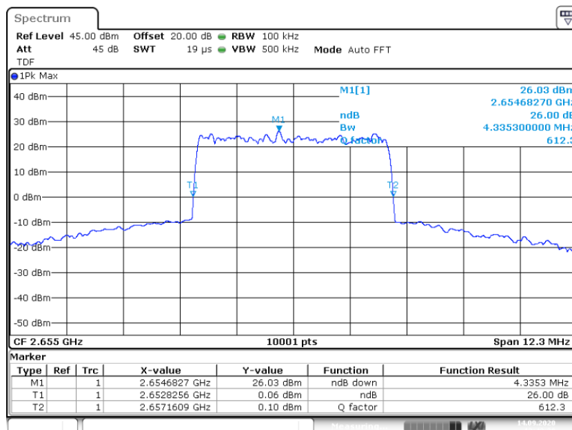
3.4 OCBw AWGN Out -0.3 2.6550G _26dB
