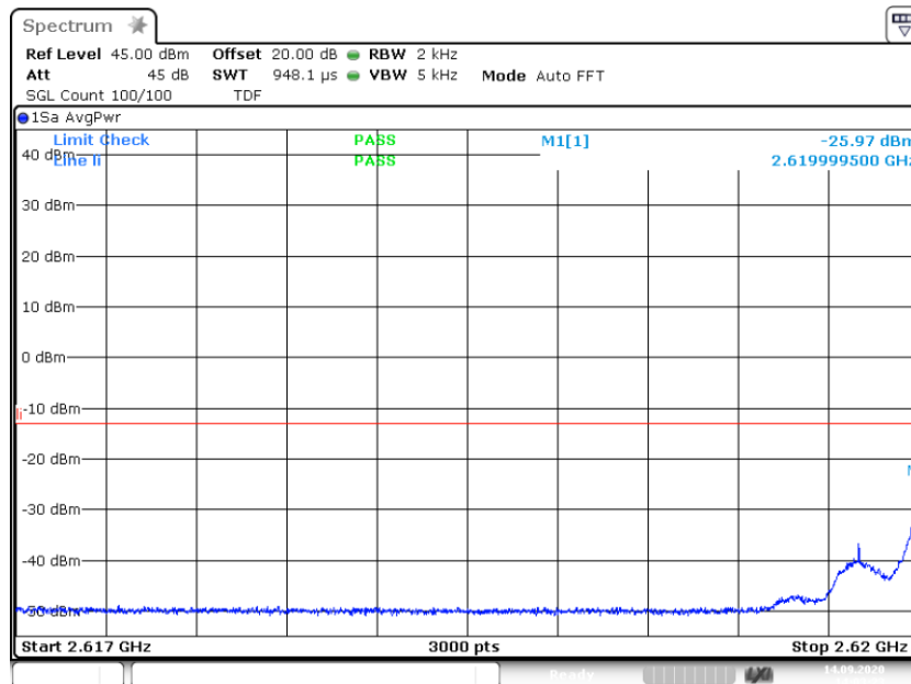
3.6.2 out of band emi IMT2600 GSM lower 2carriers -0.3 dB 2. 617G 2.620G
