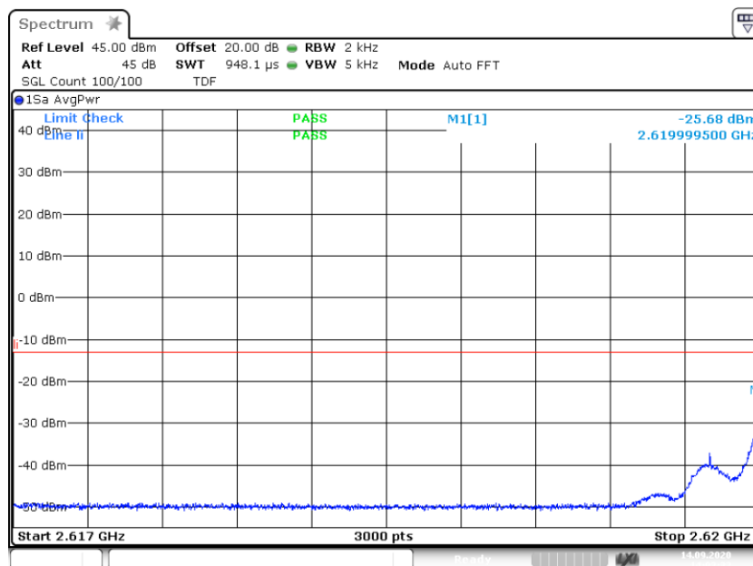
3.6.2 out of band emi IMT2600 GSM lower 2carriers +3.0 dB 2. 617G 2.620G
