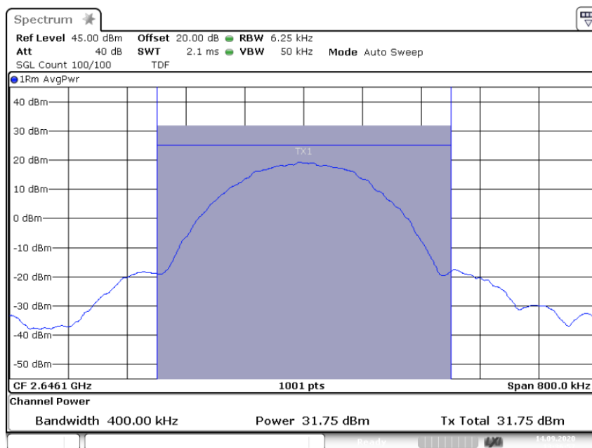
3.5.3 Power GSM Out -0.3 2.64610G
