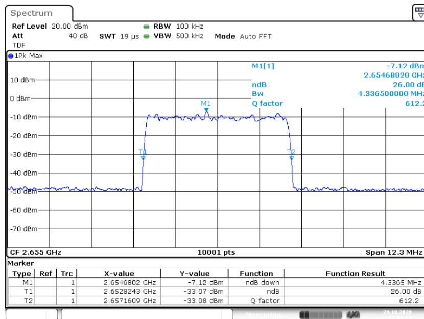
3.4 OCBw AWGN In -0.3 2.6550G _26dB
