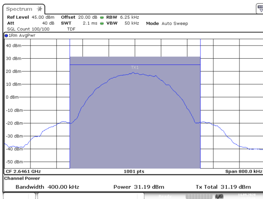
3.5.3 Power GSM Out +3 2.64610G
