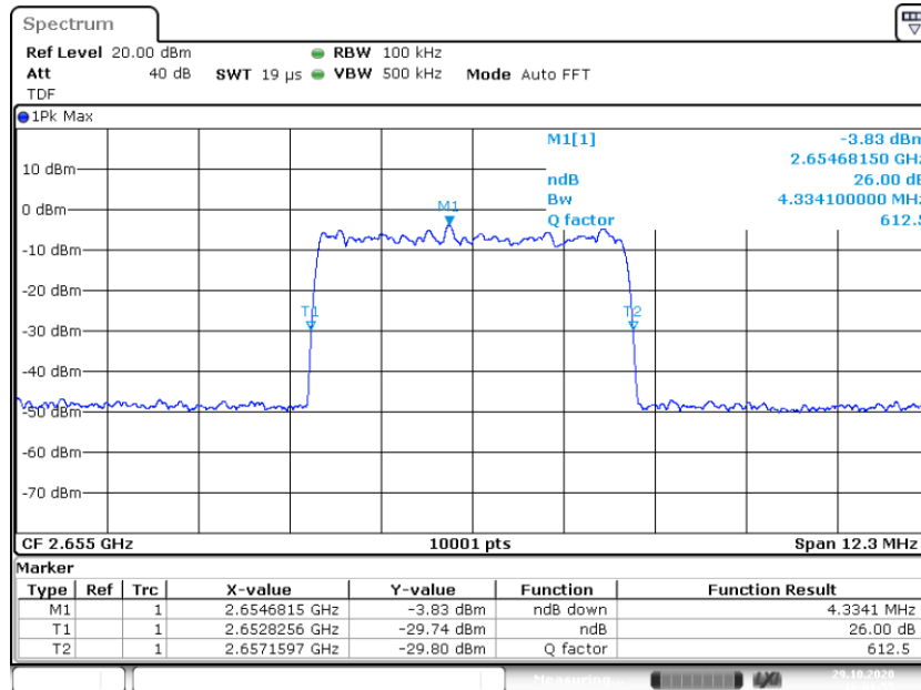
3.4 OCBw AWGN In +3 2.6550G _26dB
