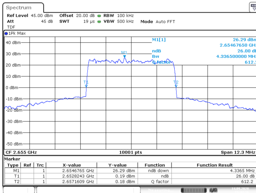
3.4 OCBw AWGN Out +3 2.6550G _26dB
