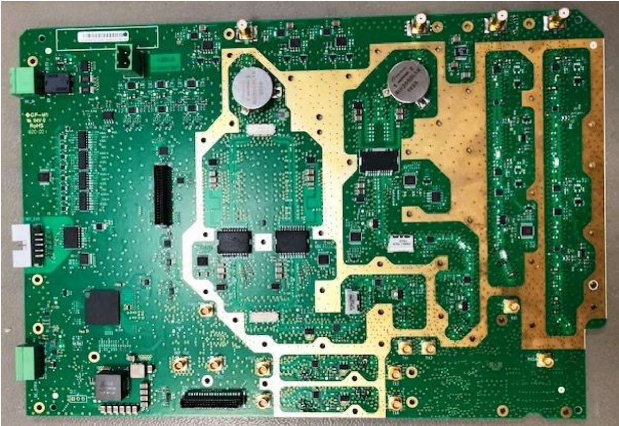
PCB P4385 CAP-M RF-1 main 17E/26 (7844263-00)
