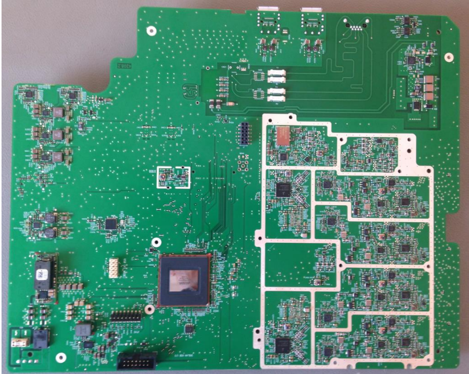
F-OTRX – Bottom view
