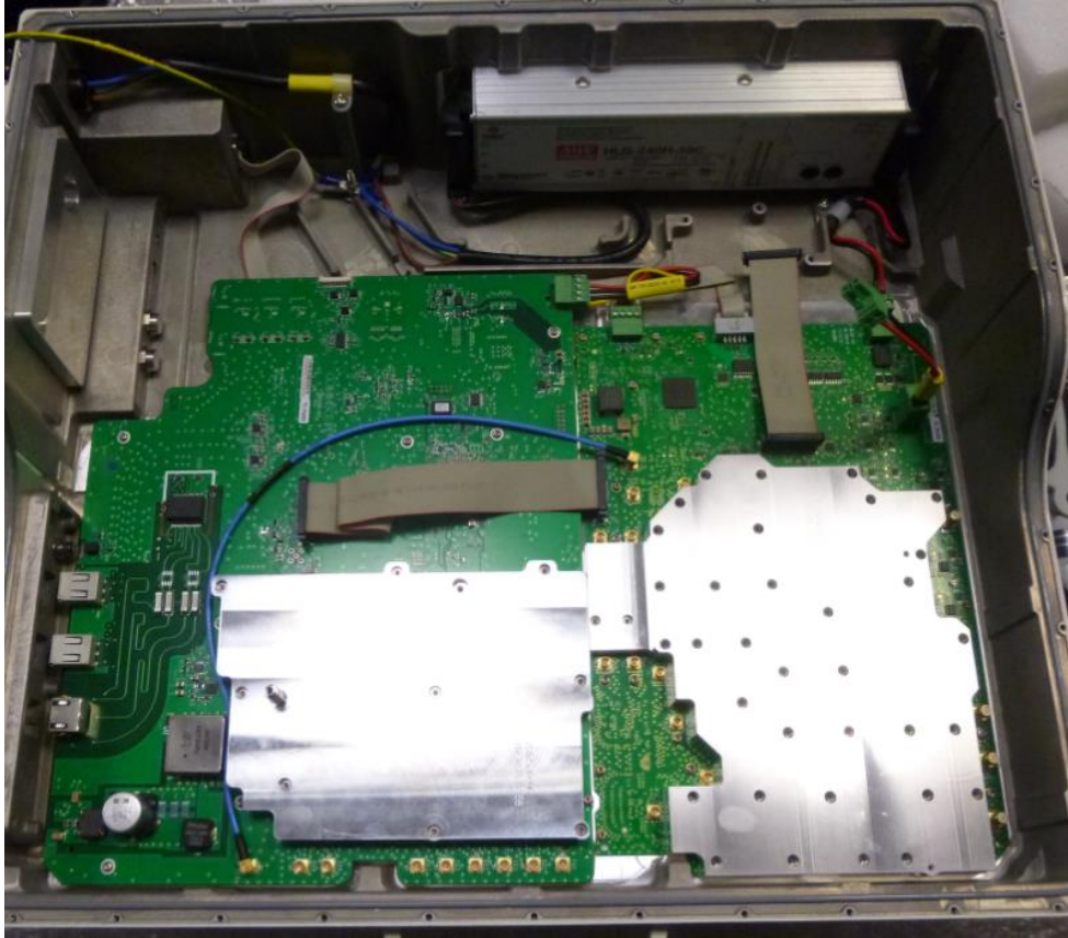
RF2 80-85/19 inside the cabinet
