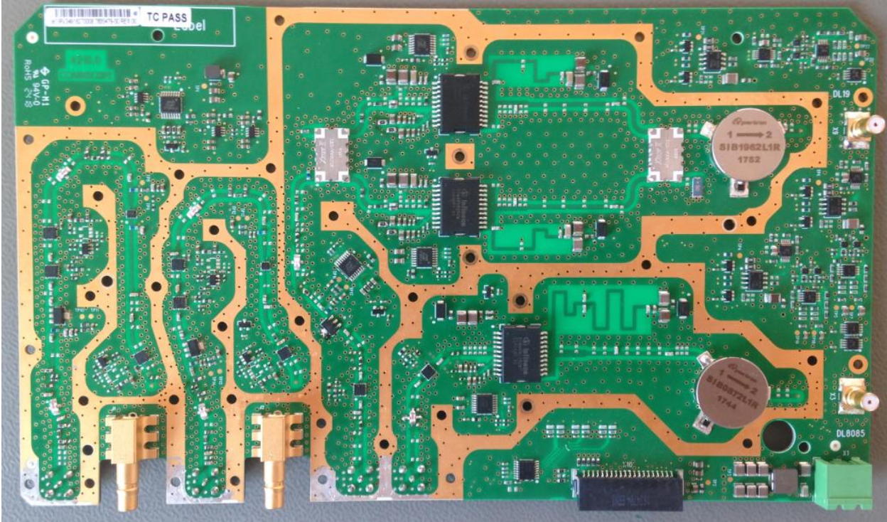
RF2 80-85/19 – Top view
