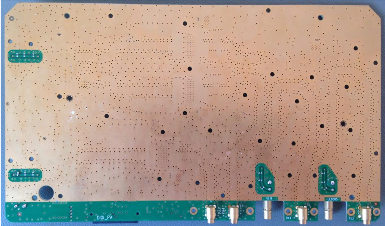
RF2 80-85/19 – Bottom view
