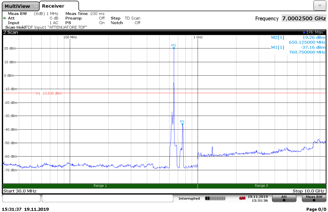
Spurious conducted emissions with input at AGC threshold at 649.5 MHz, Antenna 2
