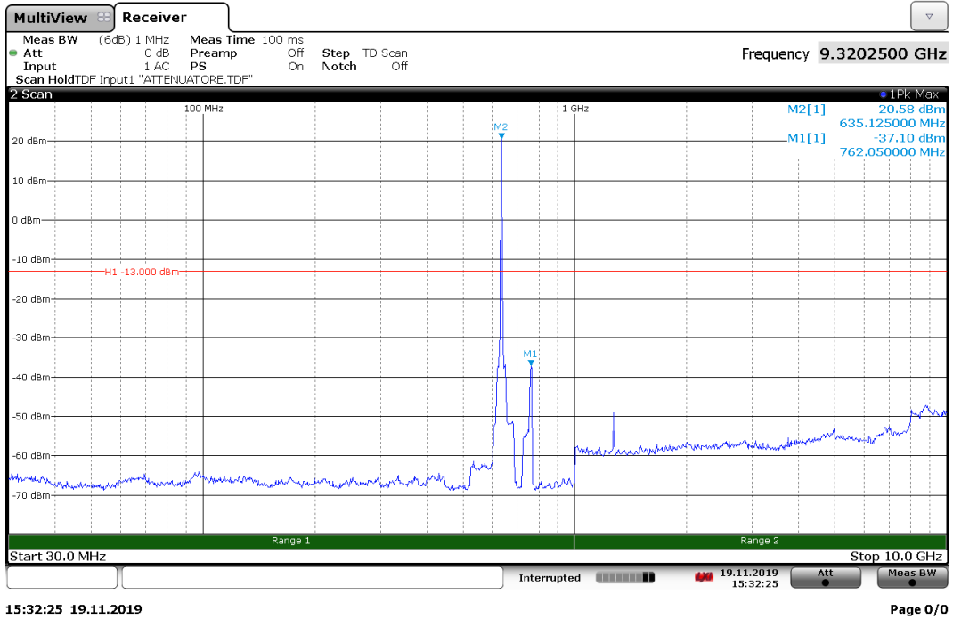
Spurious conducted emissions with input at AGC threshold at 634.5 MHz, Antenna 1
