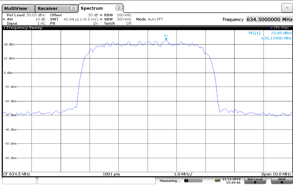
Output spectral plot with input at AGC threshold with AWGN5 signal at 634.5 MHz, Antenna 1
