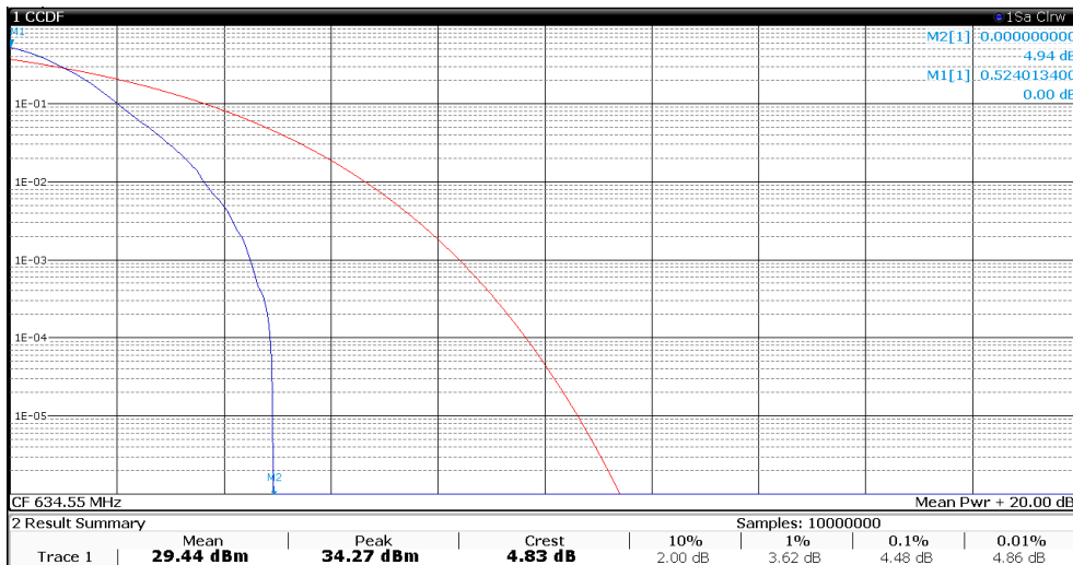
Antenna 2
