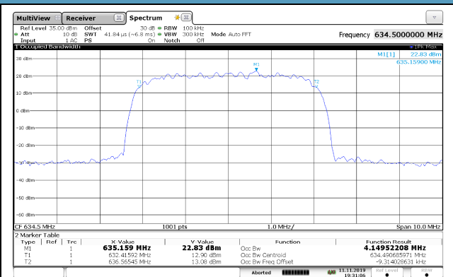
Output Antenna 1
