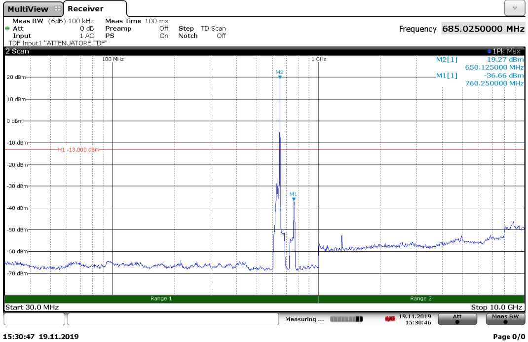
Spurious conducted emissions with input at AGC threshold at 649.5 MHz, Antenna 1
