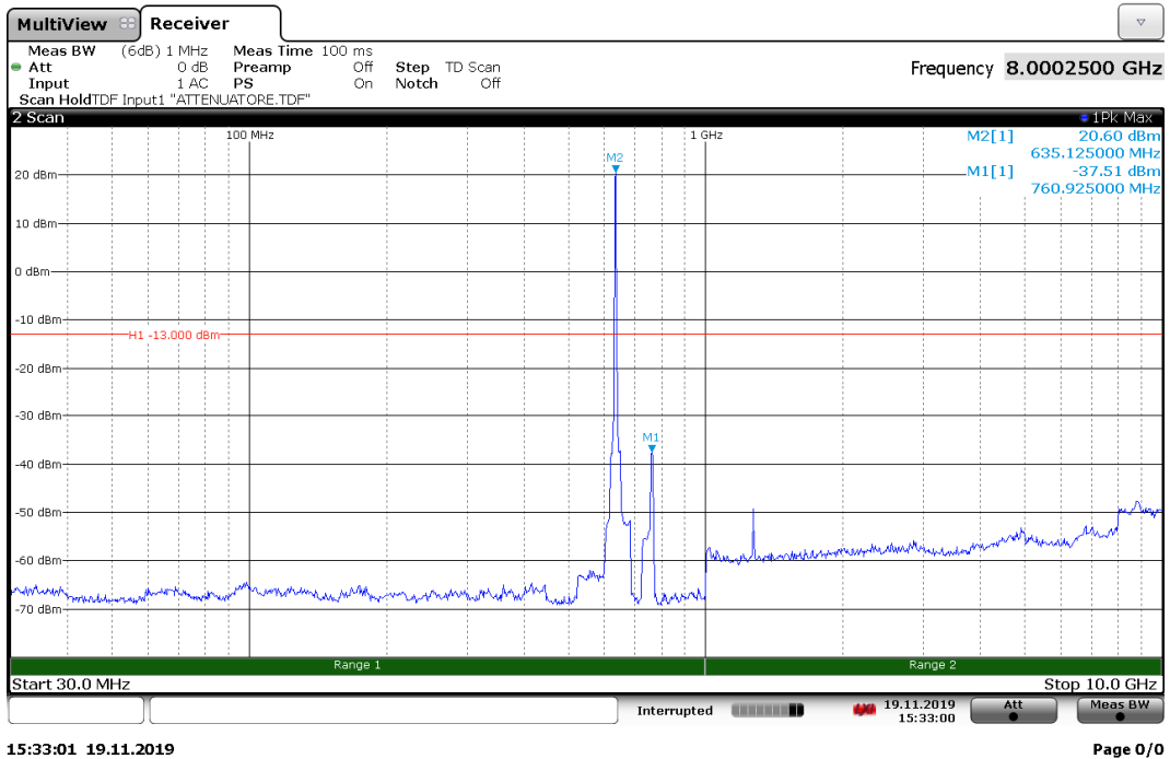
Spurious conducted emissions with input at AGC threshold at 634.5 MHz, Antenna 2
