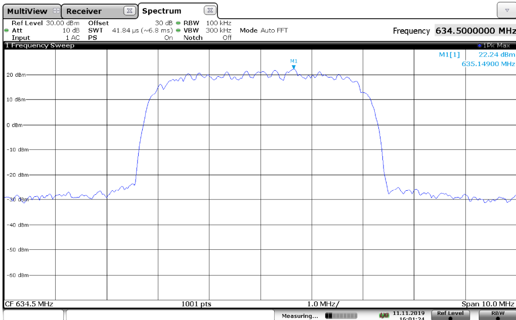
Output spectral plot with input at AGC threshold with AWGN5 signal at 634.5 MHz Antenna 2
