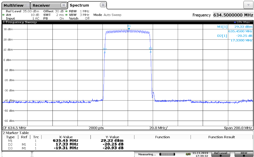
Antenna 2
