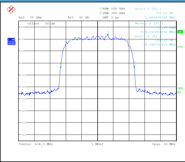
Input Output Antenna 1 26 dB bandwidth with input at AGC threshold at 634.5 MHz
