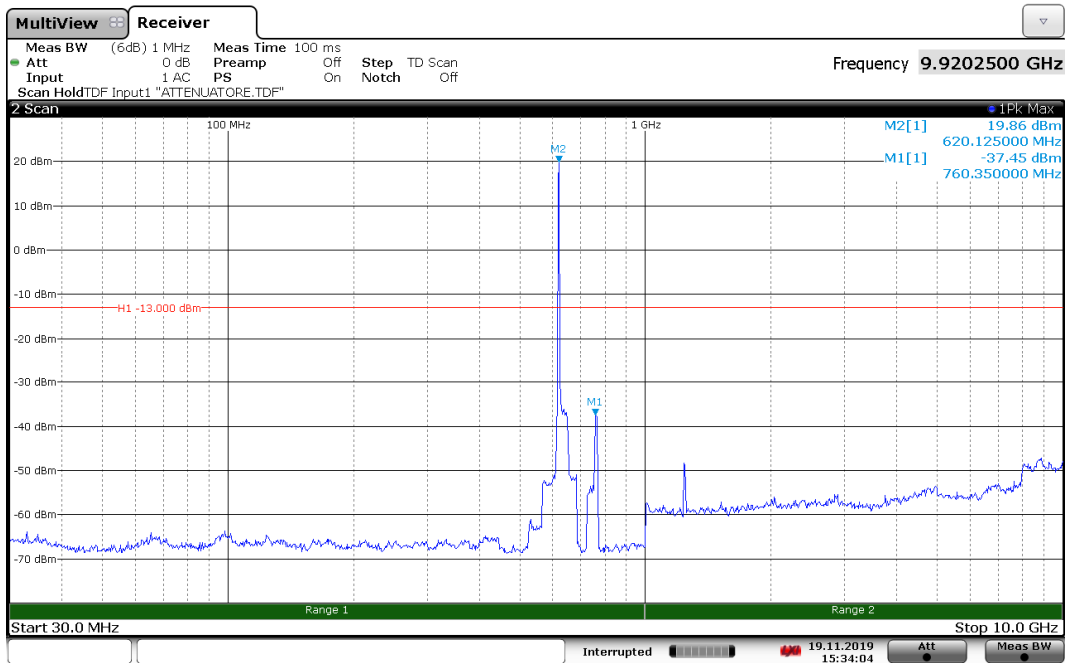
Spurious conducted emissions with input at AGC threshold at 619.5 MHz, Antenna 1
