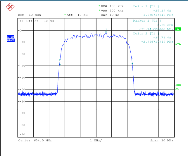
Output Antenna 1
