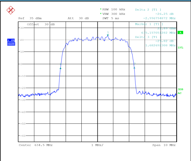
Output Antenna 2
