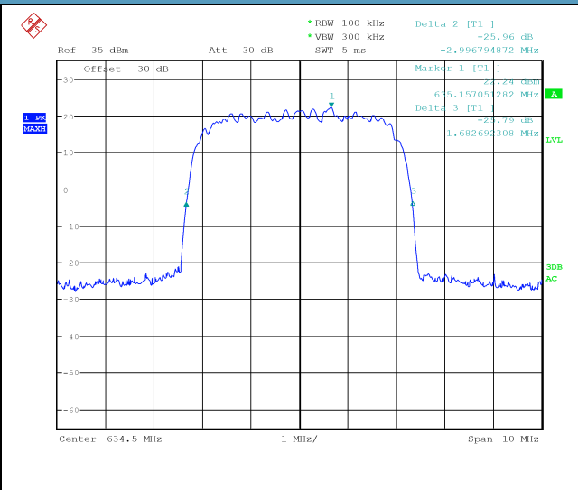
Output Antenna 2
