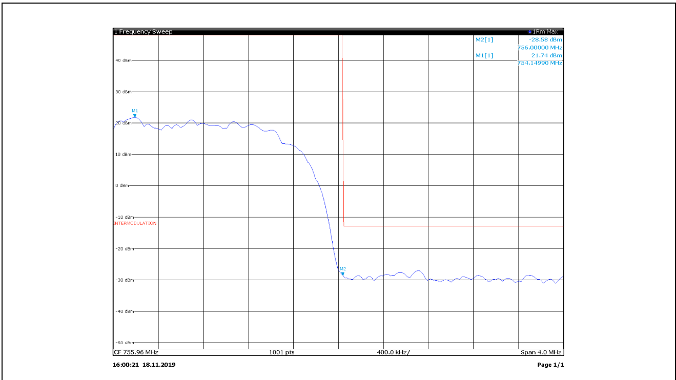
Upper block edge intermodulation products with input at AGC threshold + 3 dB, Antenna 2
