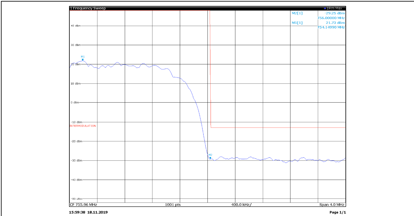
Upper block edge intermodulation products with input at AGC threshold + 3 dB, Antenna 1
