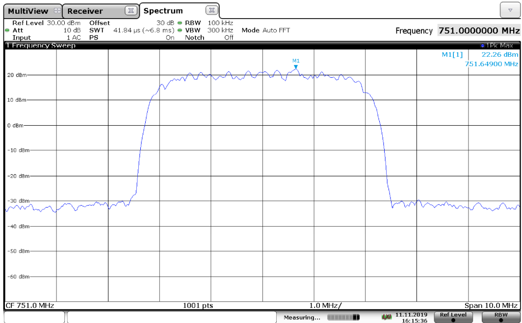
Output spectral plot with input at AGC threshold + 1 dB with AWGN5 signal at 751 MHz, Antenna 1
