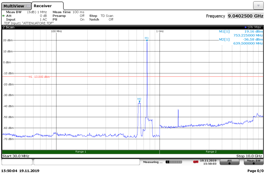
Spurious conducted emissions with input at AGC threshold at 753.5 MHz, Antenna 1
