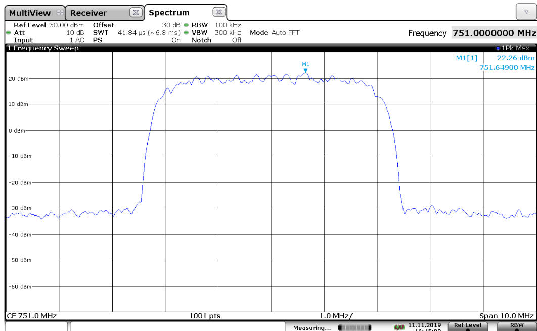
Output spectral plot with input at AGC threshold with AWGN5 signal at 751 MHz, Antenna 1
