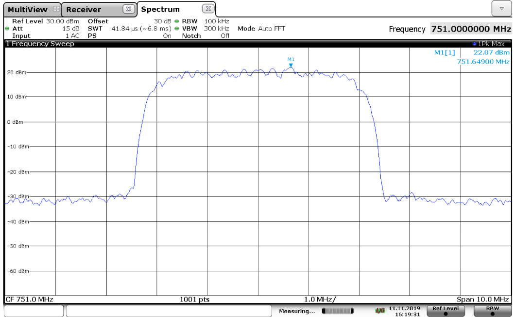
Output spectral plot with input at AGC threshold + 1 dB with AWGN5 signal at 751 MHz, Antenna 2
