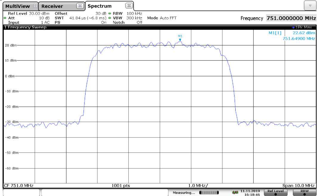
Output spectral plot with input at AGC threshold with AWGN5 signal at 751 MHz, Antenna 2
