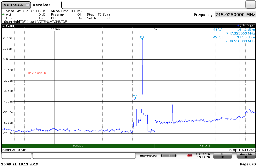
Spurious conducted emissions with input at AGC threshold at 748.5 MHz, Antenna 2
