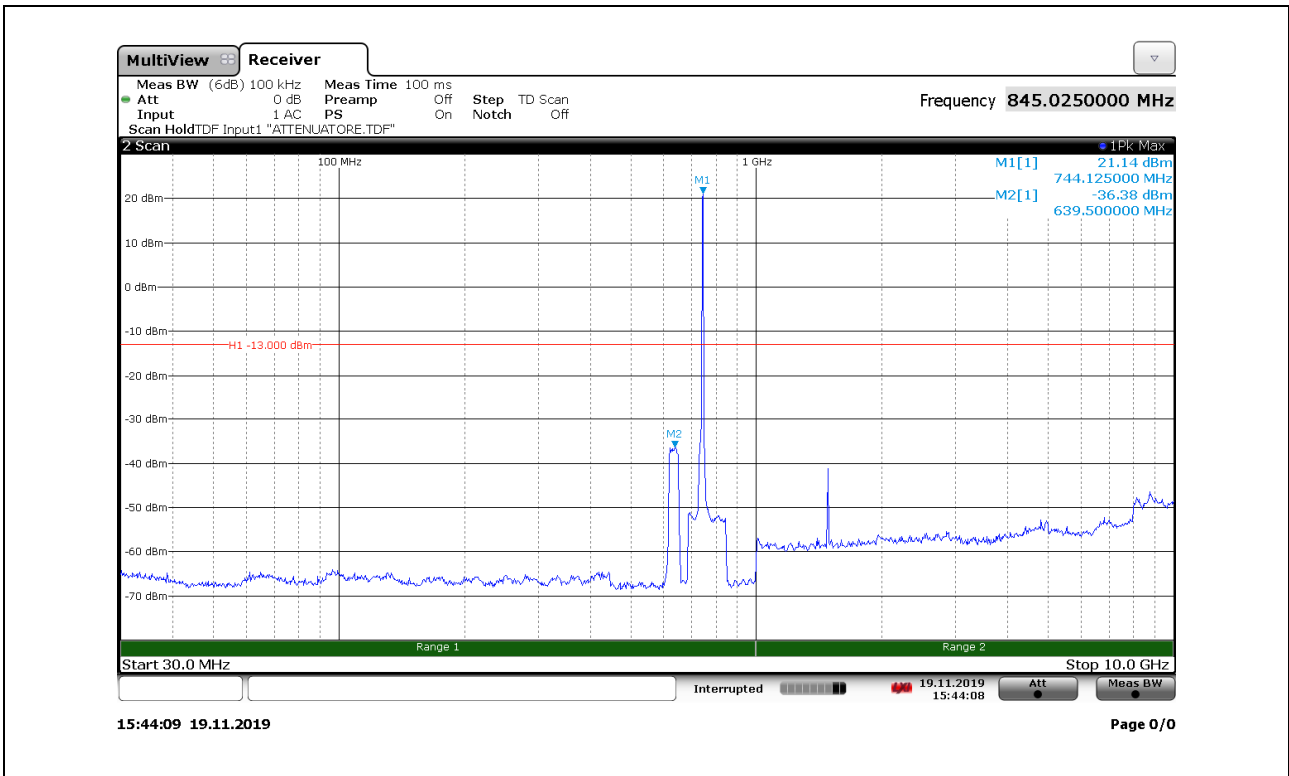
Spurious conducted emissions with input at AGC threshold at 743.5 MHz, Antenna 1
