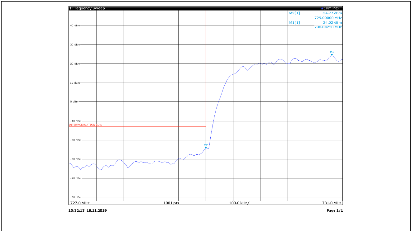
Lower block edge with input at AGC threshold, Antenna 2
