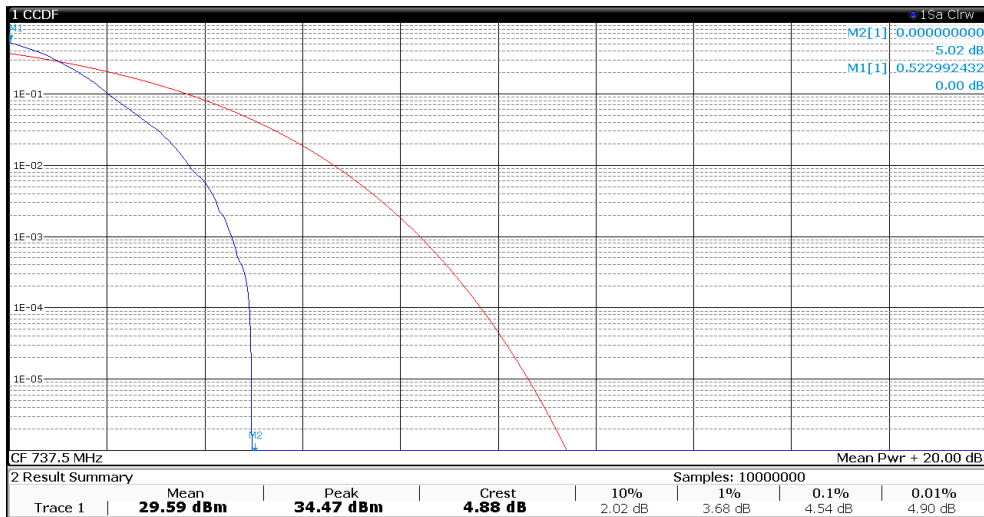
Antenna 2
