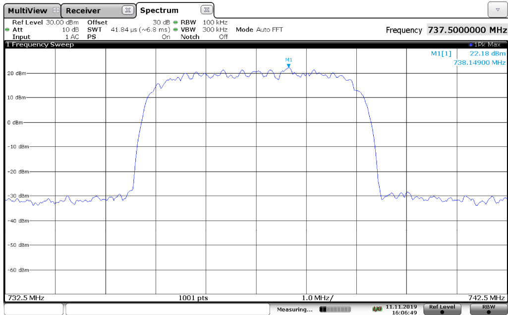
Output spectral plot with input at AGC threshold + 1 dB with AWGN5 signal at 737.5 MHz, Antenna 2
