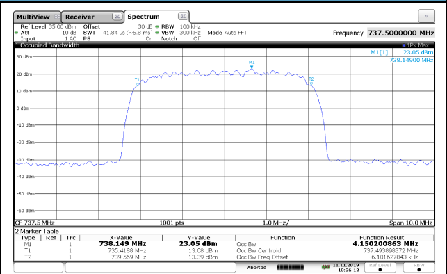
Output Antenna 1
