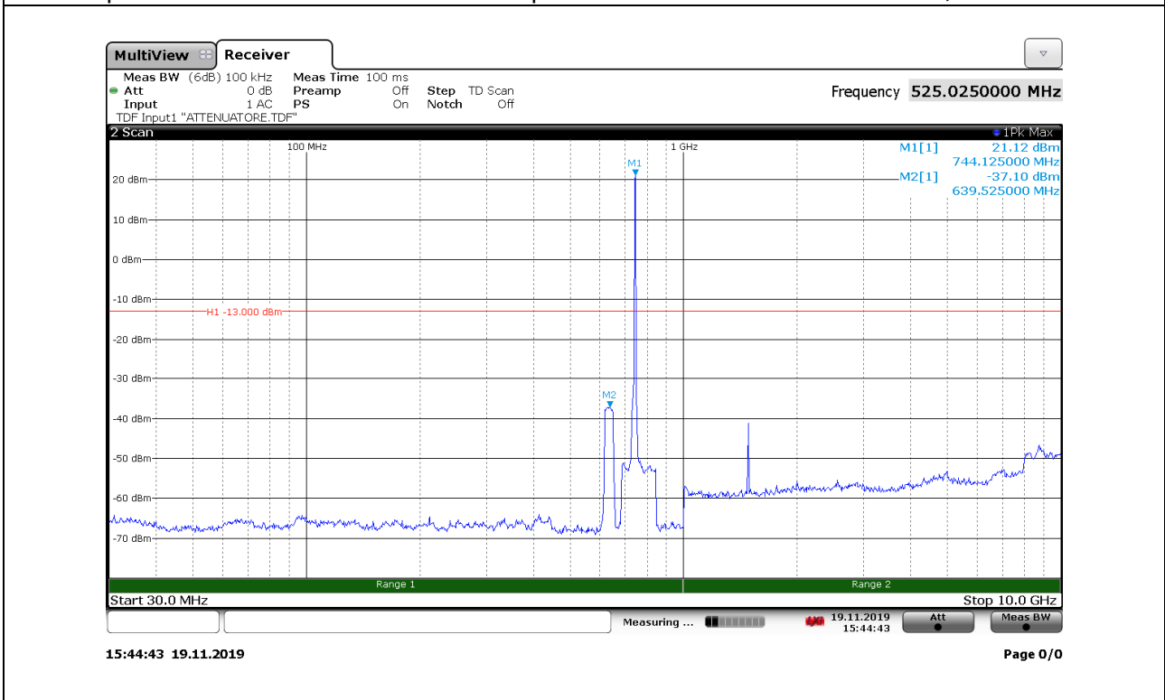
Spurious conducted emissions with input at AGC threshold at 743.5 MHz, Antenna 2
