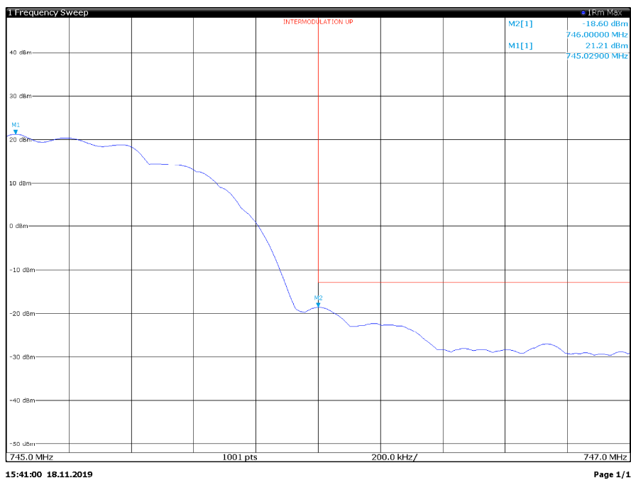
Upper block edge intermodulation products with input at AGC threshold + 3 dB, Antenna 1
