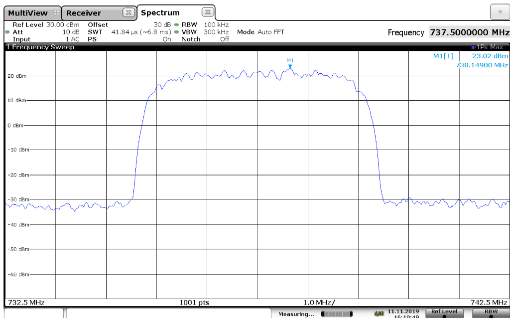
Output spectral plot with input at AGC threshold with AWGN5 signal at 737.5 MHz, Antenna1
