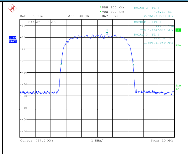
Output Antenna 2
