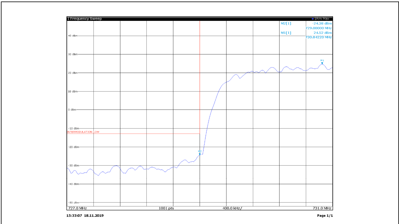
Lower block edge with input at AGC threshold + 3 dB, Antenna 1
