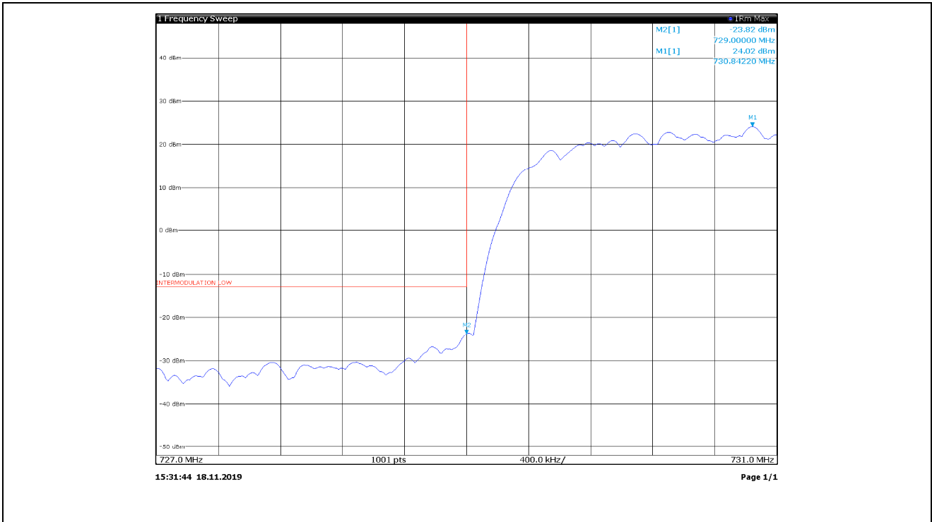
Lower block edge with input at AGC threshold, Antenna 1
