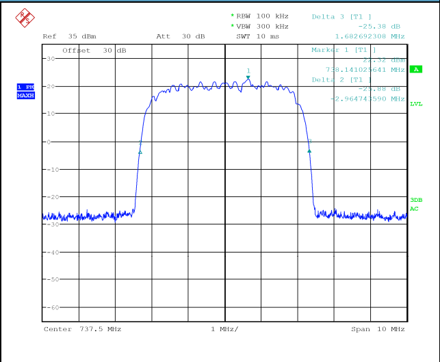
Output Antenna 2
