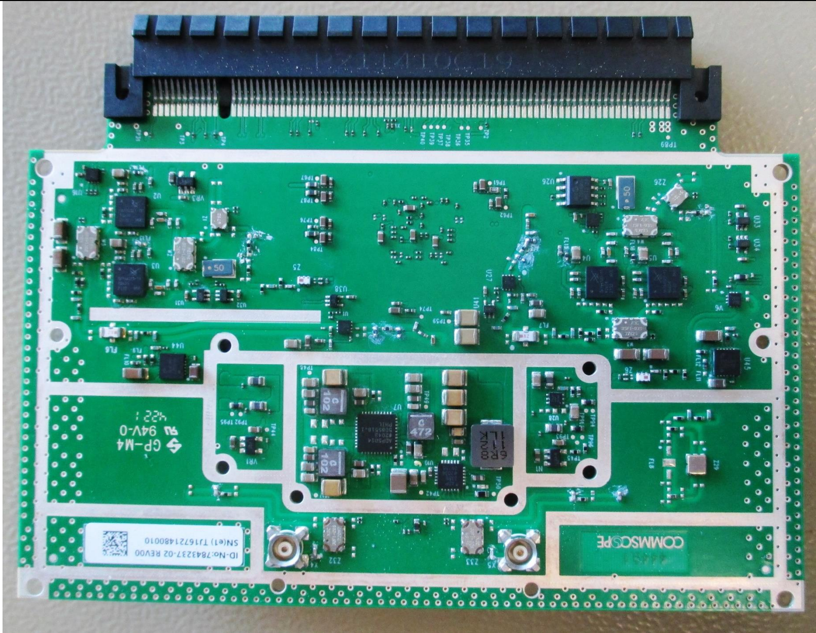
7843237-02 P4449 C-Band WB RM CAP L2
