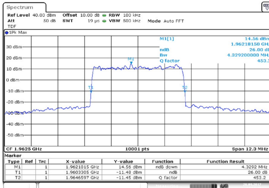
Output Signal
