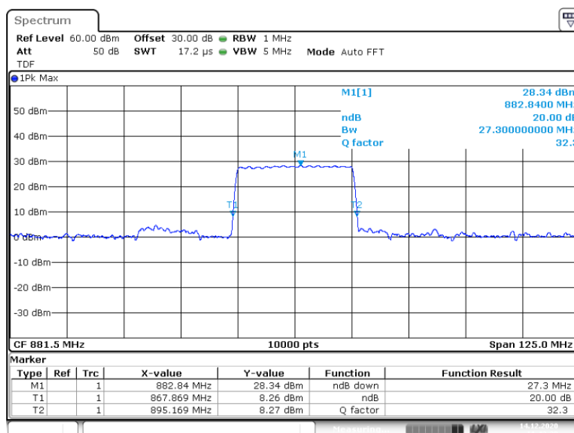
3.3 Out of band rejection Band 5 881.50000M _20dB
