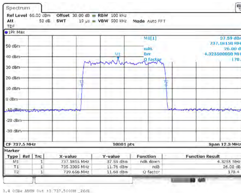
Output Signal
