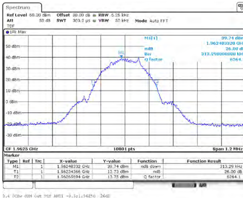
Output Signal
