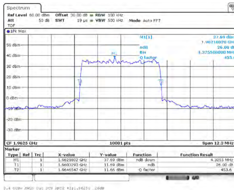
Output Signal
