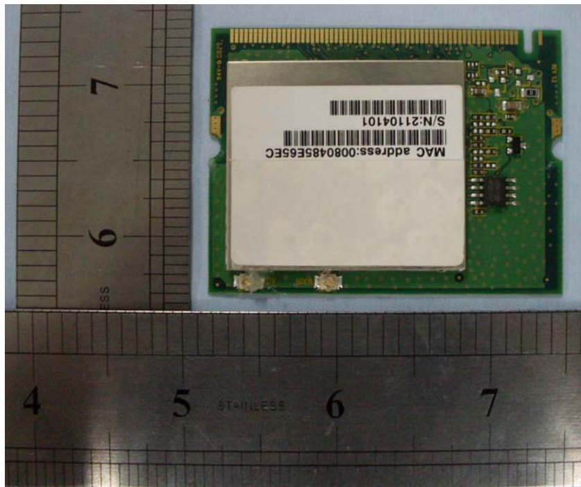
Wifi module PCB 1 view
