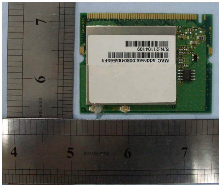
Wifi module PCB 2 view
