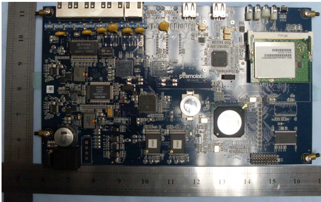
PCB view
