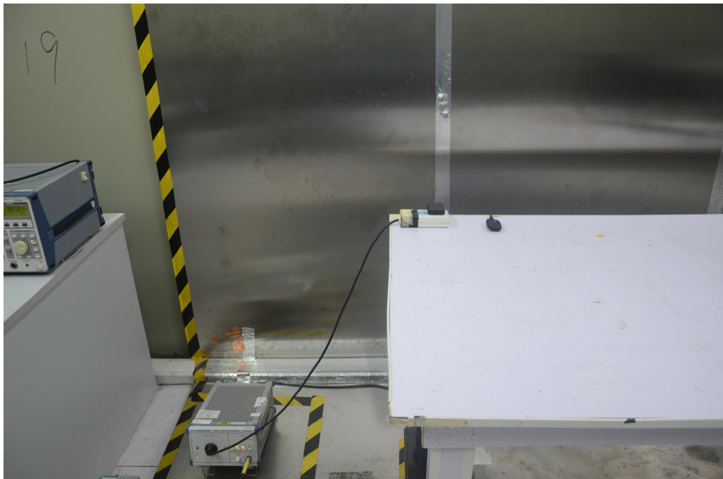
Conducted Emissions
