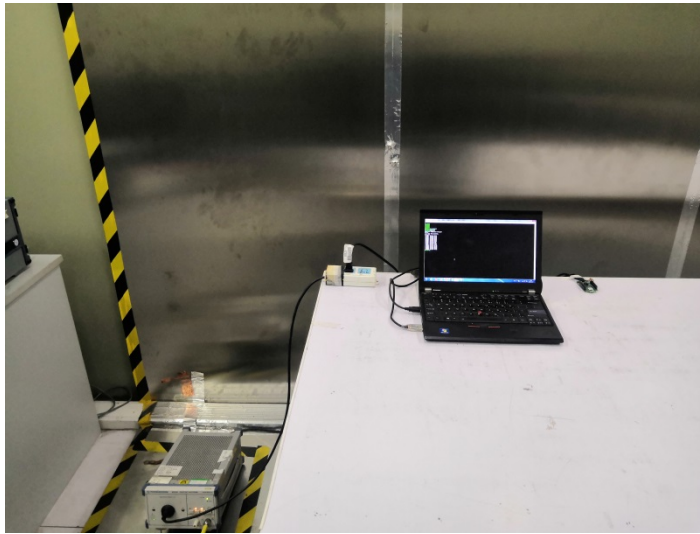
Conducted Emission
