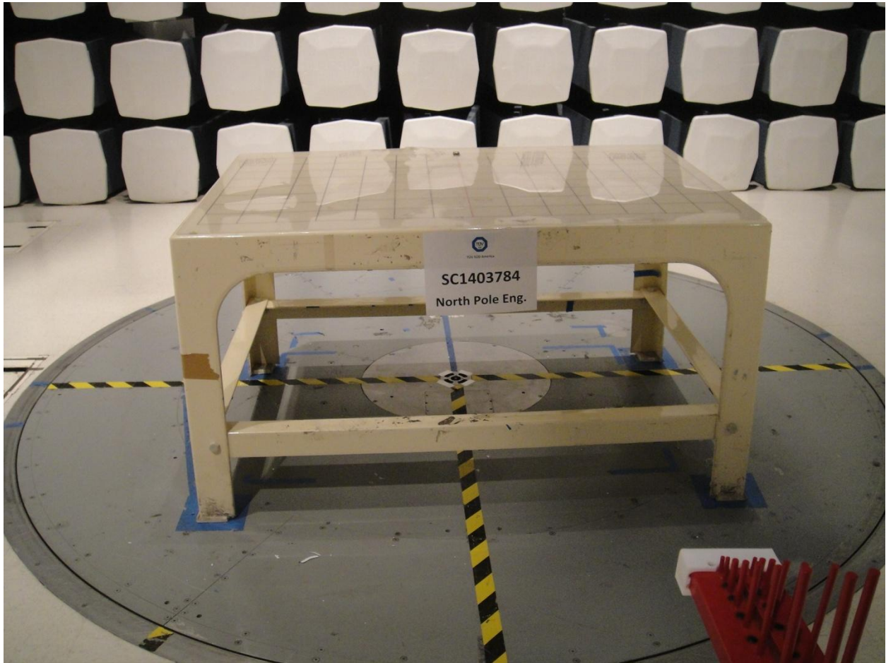
Radiated Emission Below 1GHz (Front)
