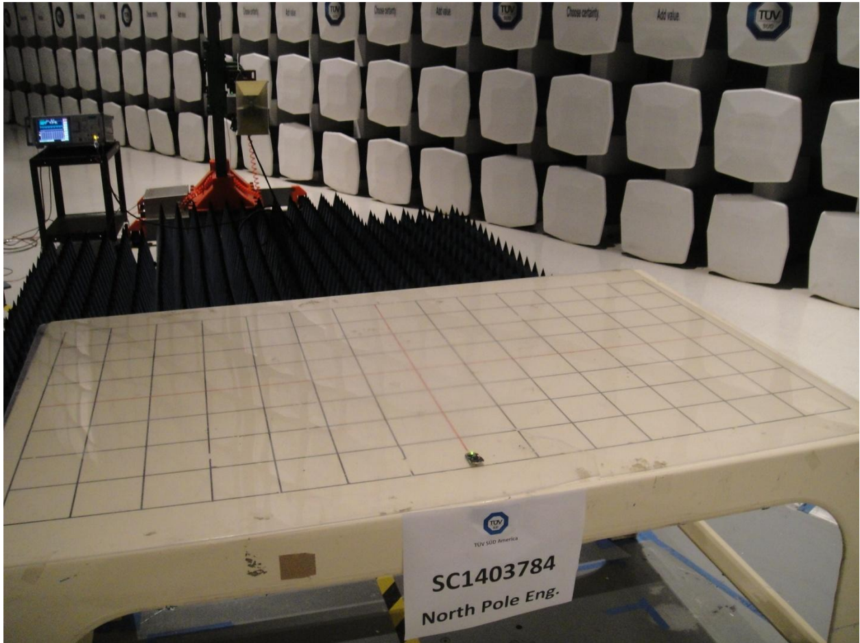
Radiated Emission Above 1GHz (Back)
