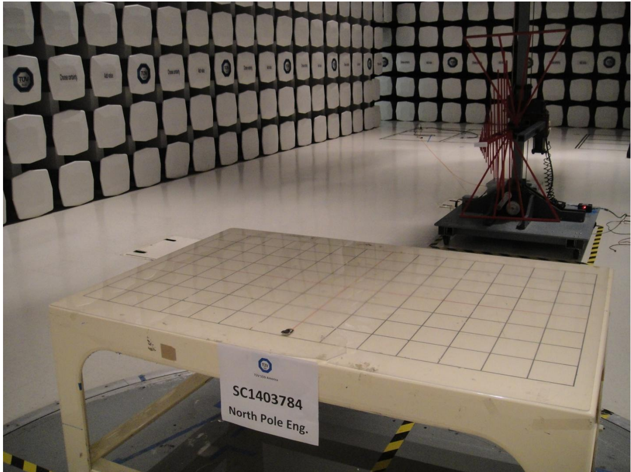
Radiated Emission Below 1GHz (Back)
