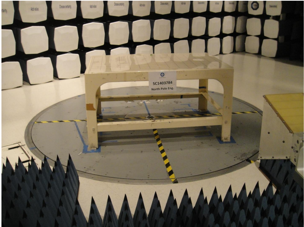
Radiated Emission Above 1GHz (Front)
