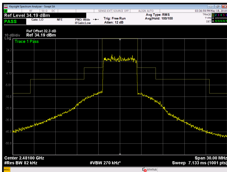
Figure 20 - Top Channel - Transmitter Mask - 5 MHz Bandwidth, Port A
