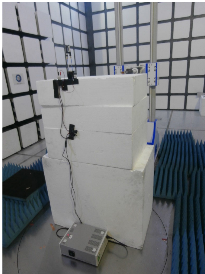
Radiated Emissions 18 GHz to 30 GHz
