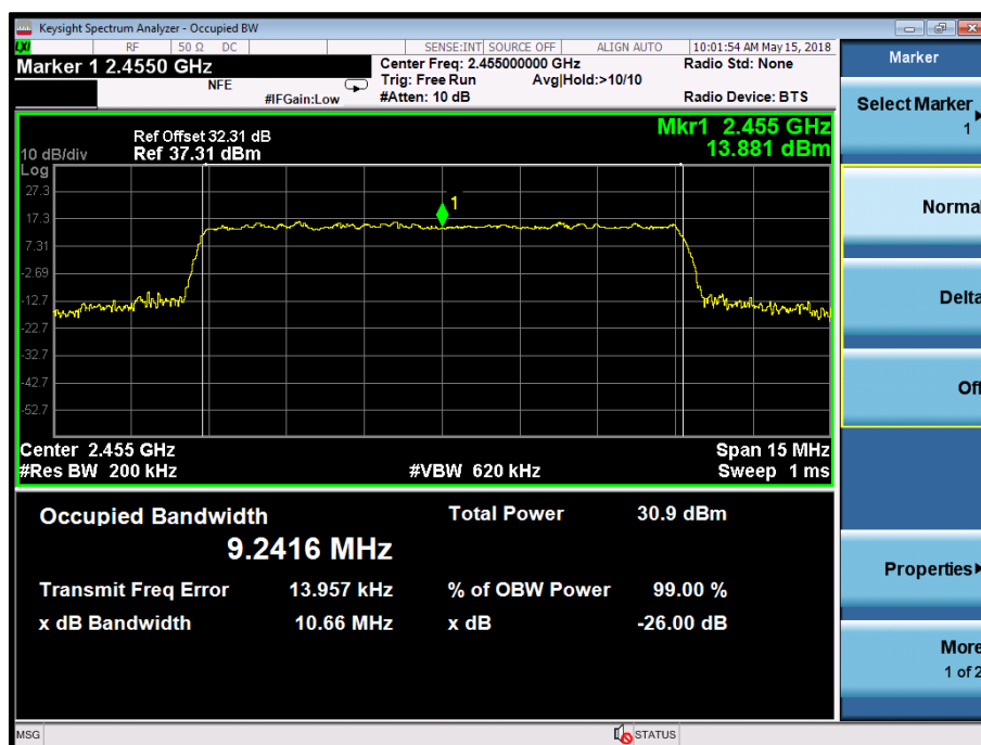
Figure 8 - Bottom Channel - Occupied Bandwidth - 10 MHz Bandwidth, Port A
