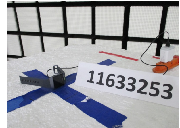
ANTENNA AT Y POSITION FRONT PHOTO
