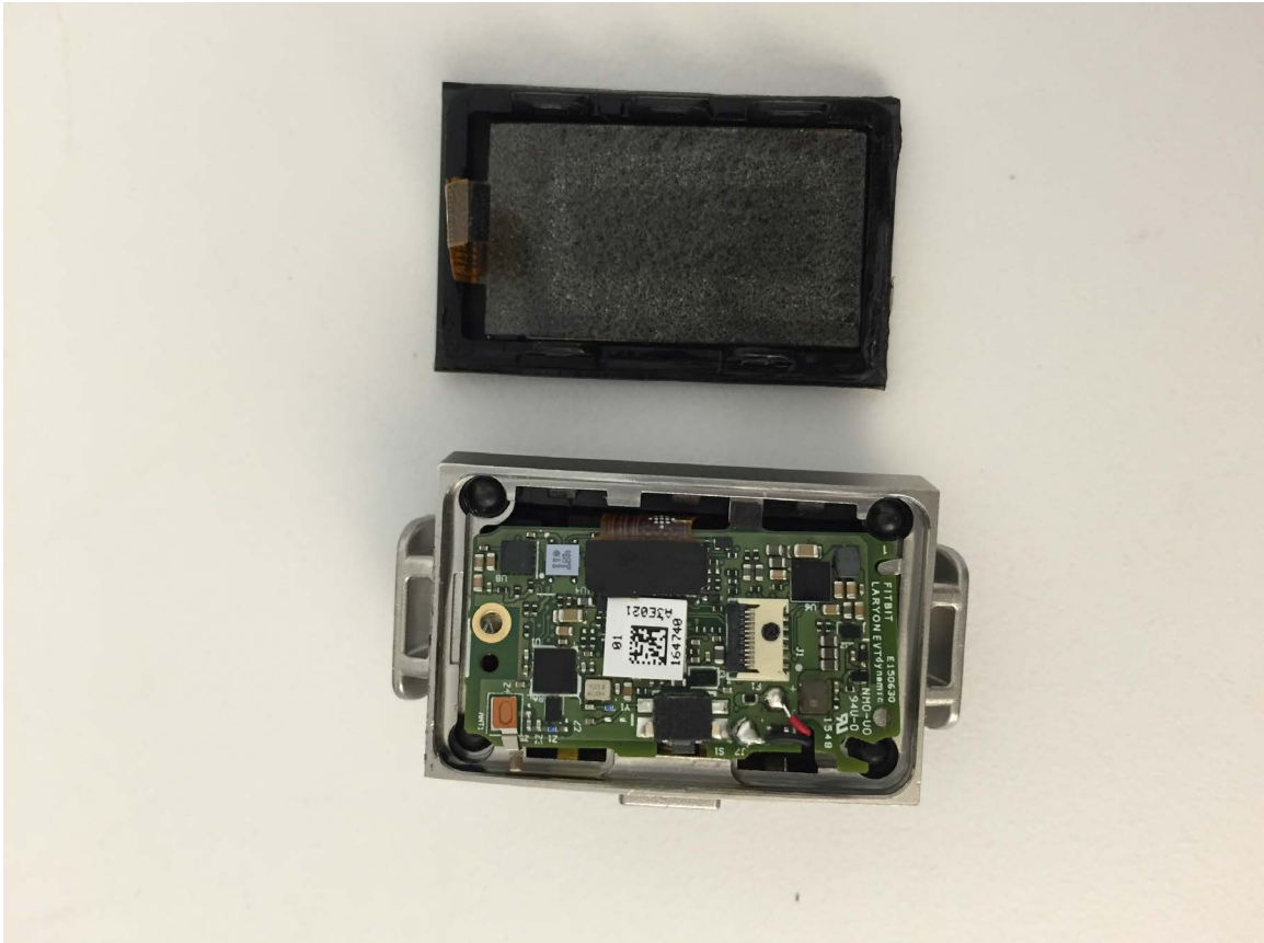
PCB TOP VIEW #1
