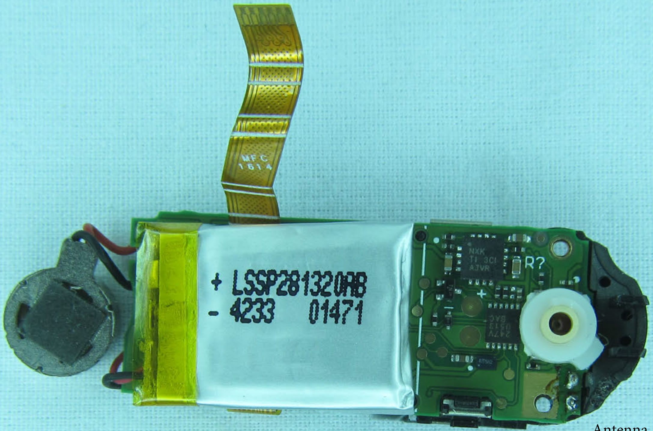
Antenna connectors
