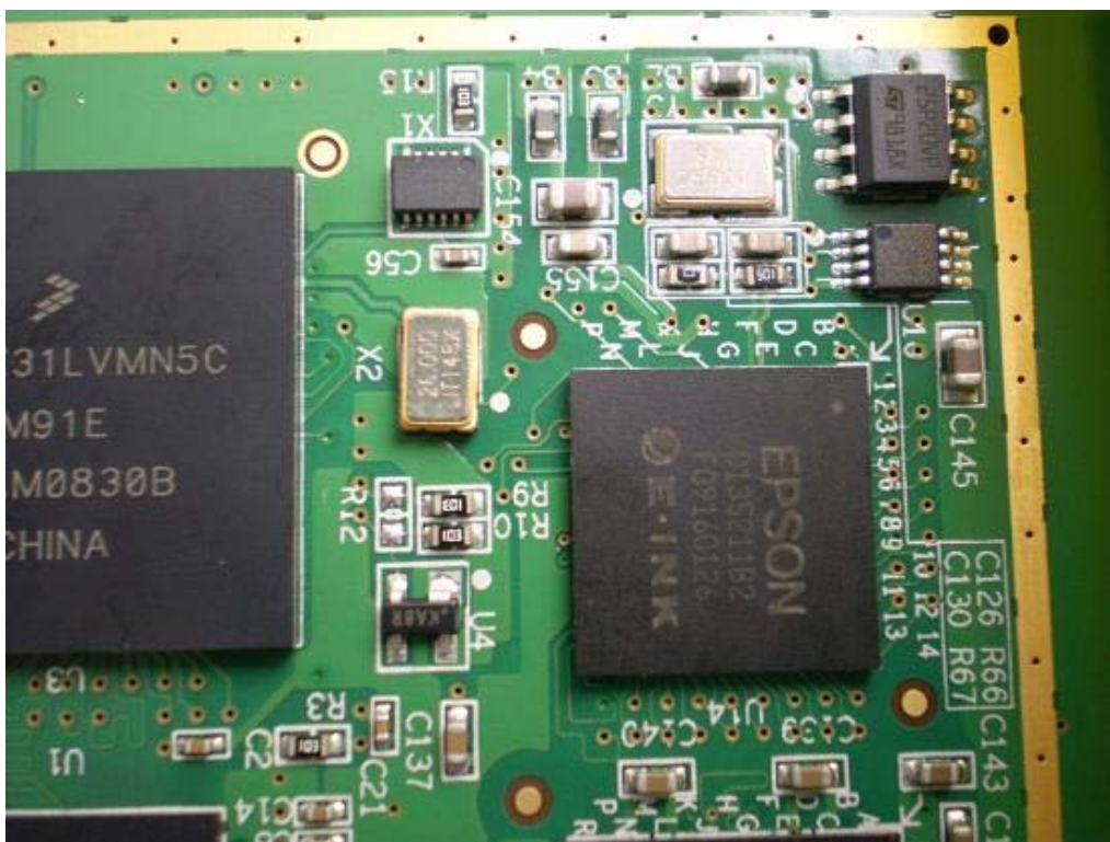
(5. Epson/E-ink S1D13521 Display Controller)
