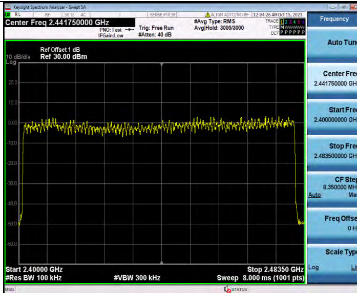
8DPSK Modulation
