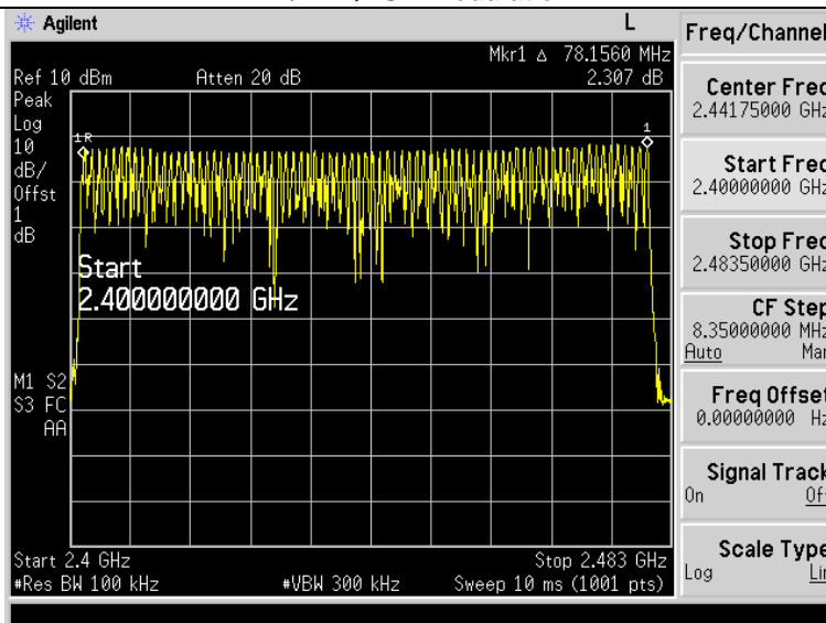
8DPSK Modulation
