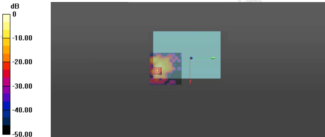
0 dB = 0.60 W/kg
