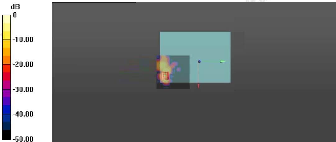
0 dB = 0.58 W/kg
