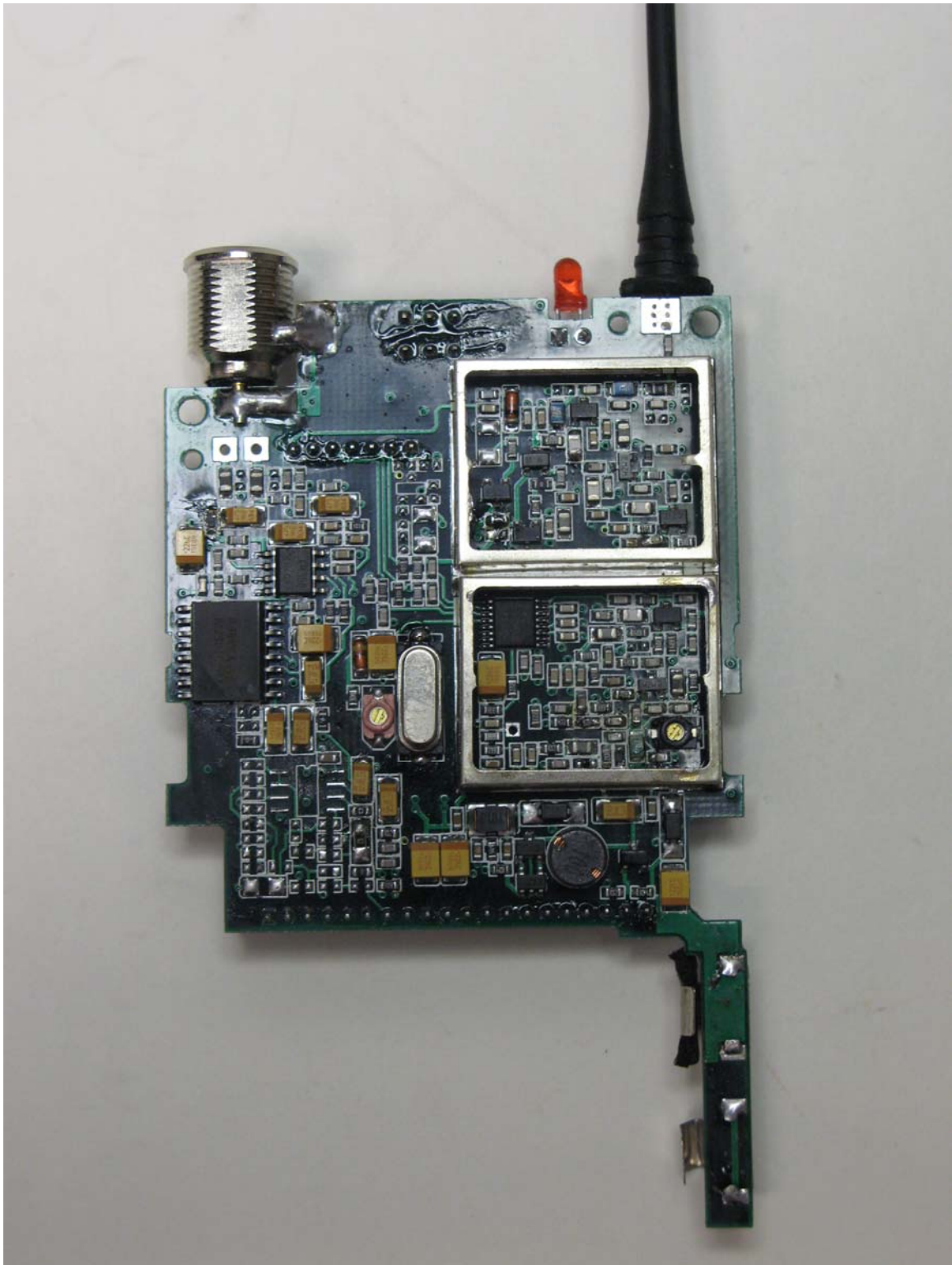
Passport Executive – View of PCB RF side (shields removed)
