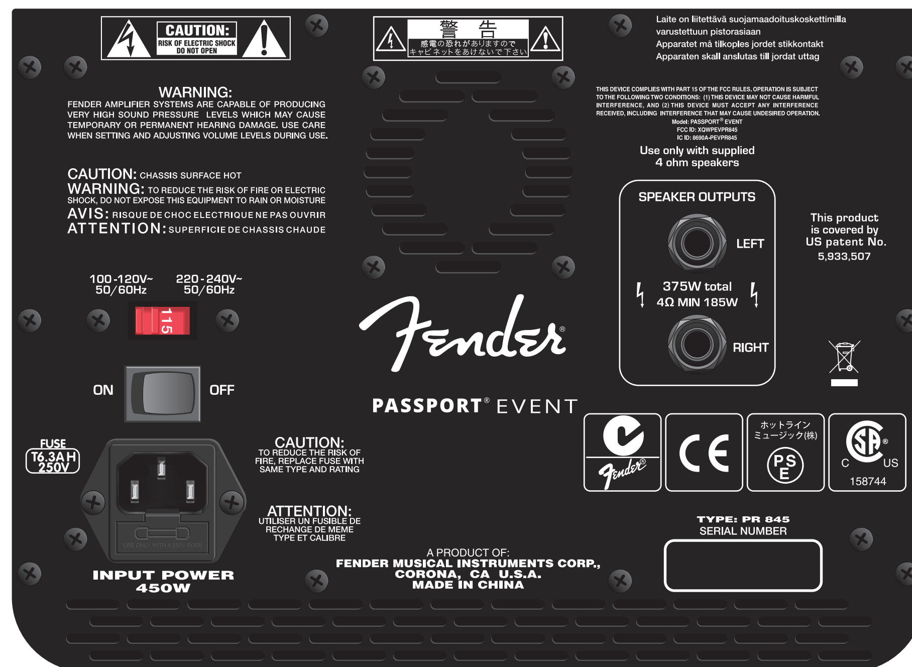
PANEL REAR PASSPORT EVENT 2712CGP002 REV 4.2
