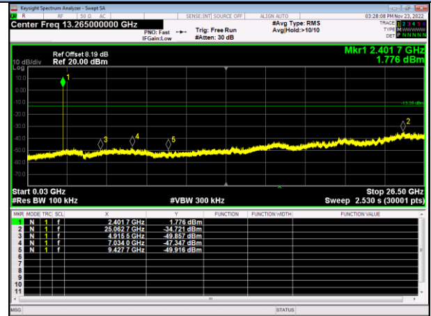
2Mbps / Mid Channel / 30MHz~26.5GHz
