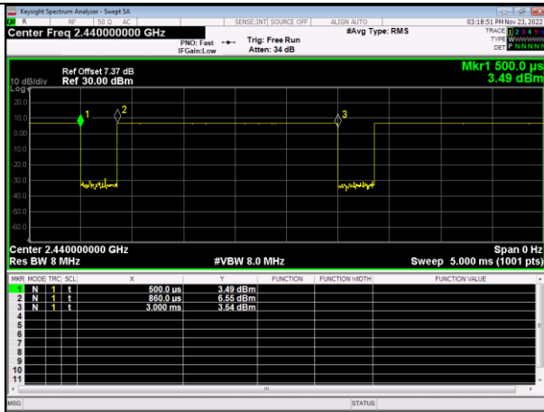
TP time
