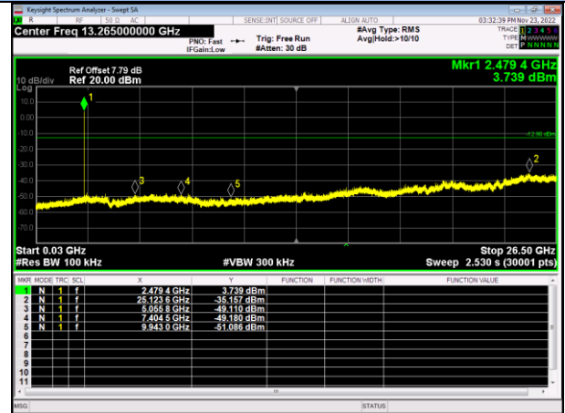
2Mbps / High Channel / 30MHz~26.5GHz
