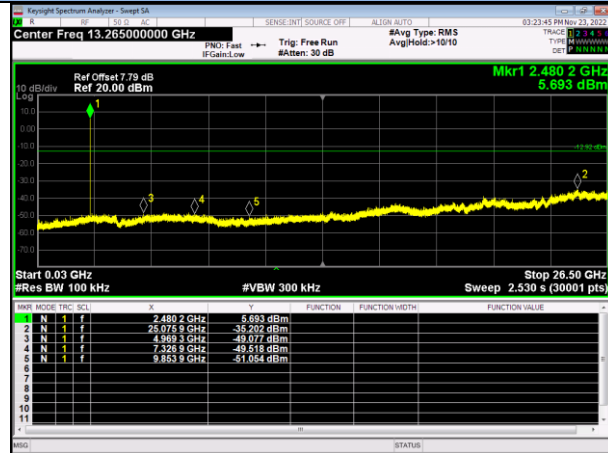
1Mbps / High Channel / 30MHz~26.5GHz
