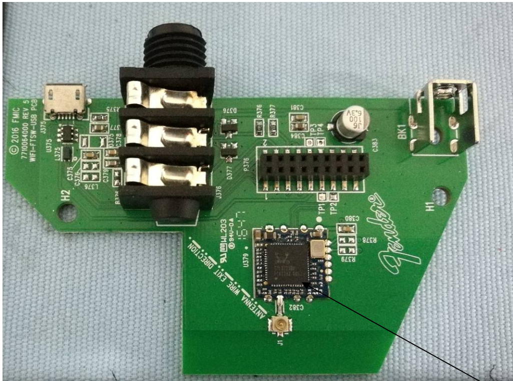
RF Chip
