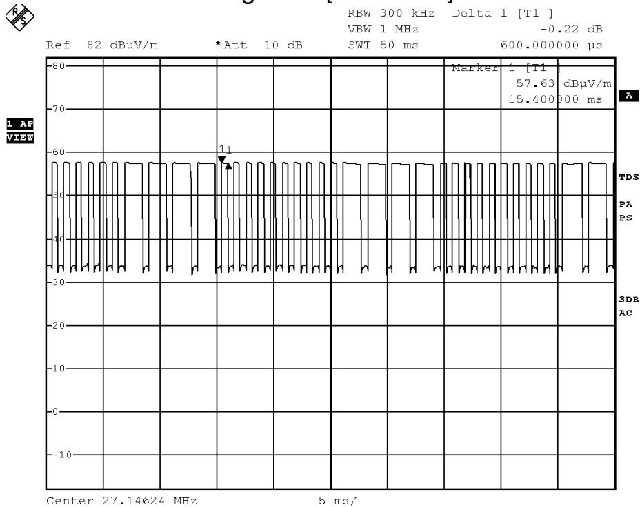
Figure C [Short Pulse]
