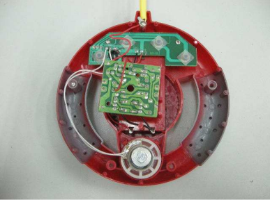
Front View of the product (Internal)
