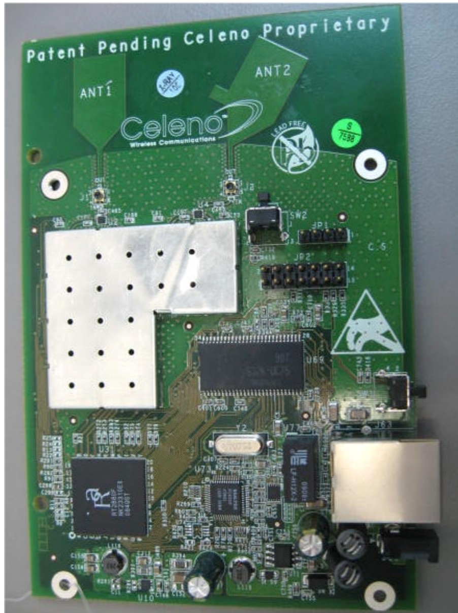
Photograph No4 Client printed circuit board front view
