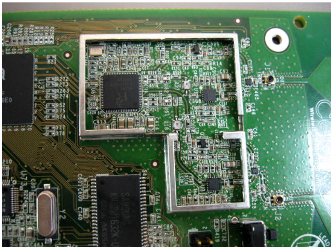
Photograph No6 RF module without shields
