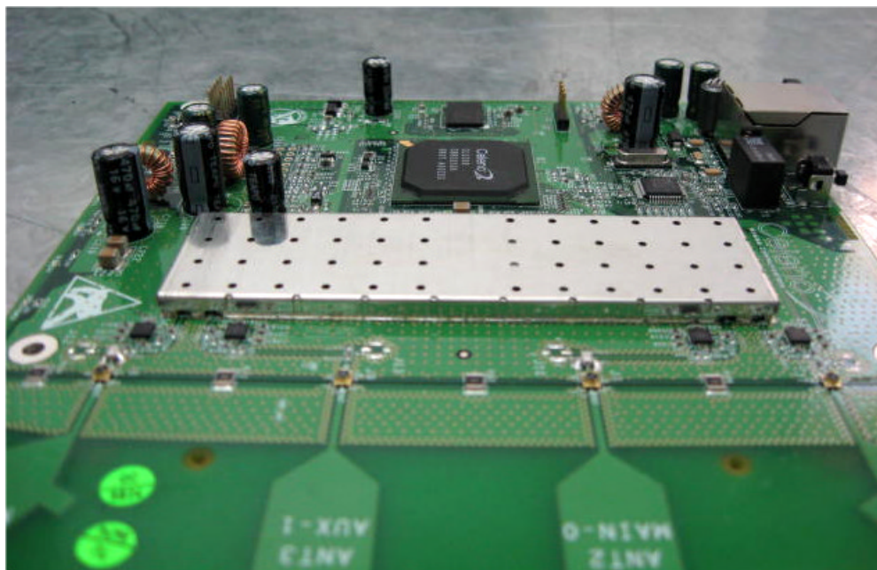
Photograph No.5 RF module
