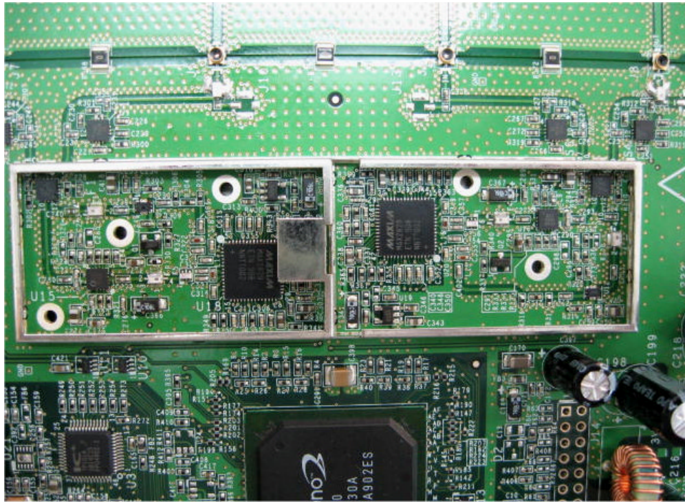
Photograph No6 RF module without shields
