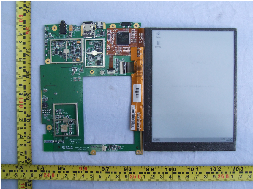
PCB without Shield Front View
