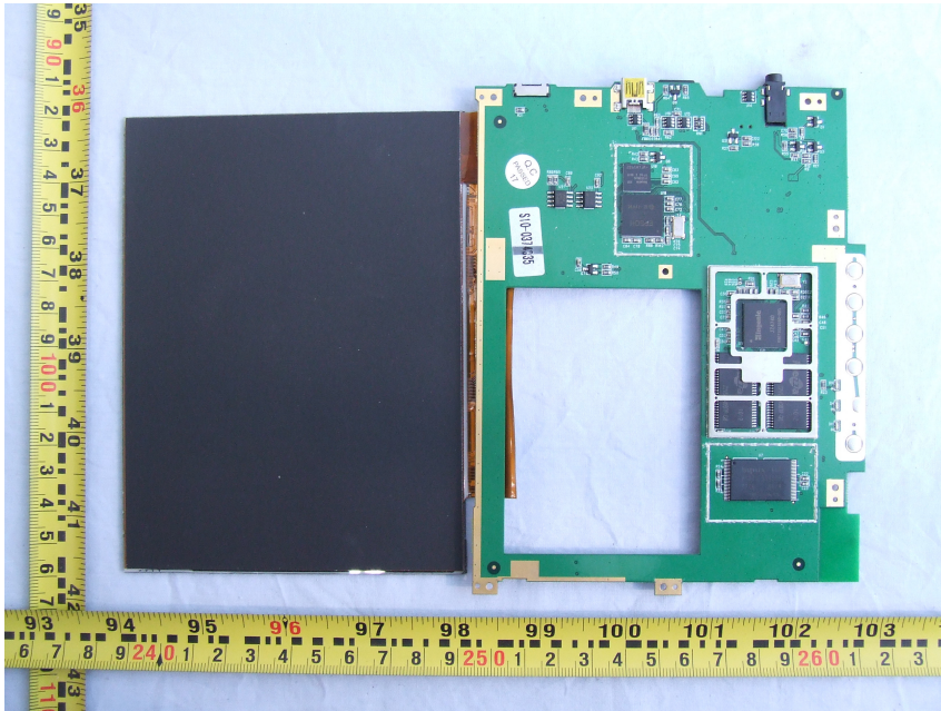
PCB without Shield Rear View
