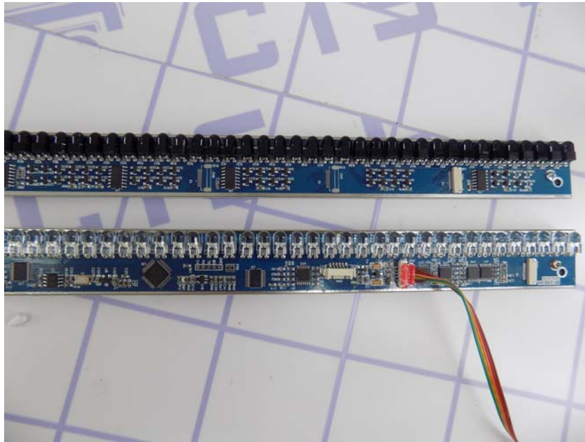
PCB – Part 11 view
