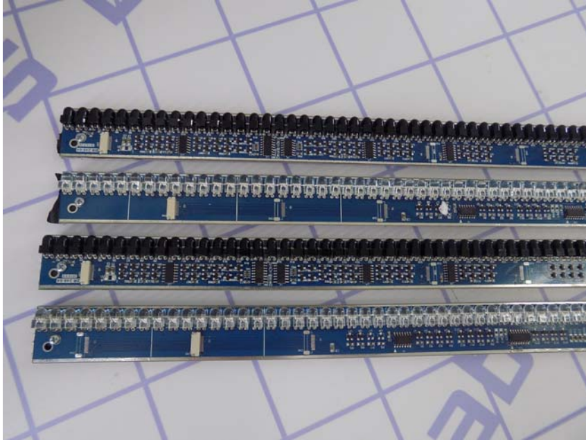
PCB- Part 1 view
