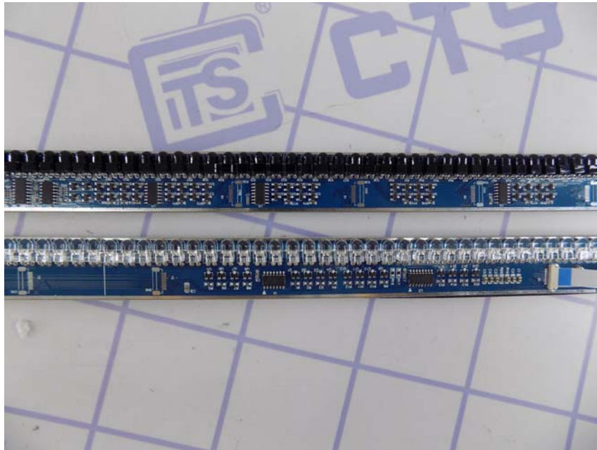
PCB – Part 9 view
