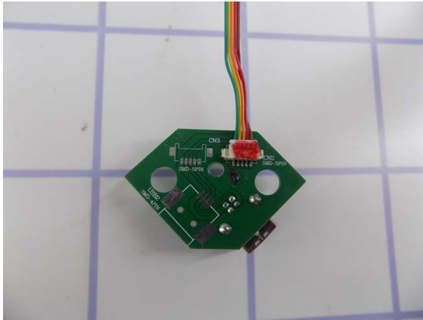
USB – PCB side 2 view
