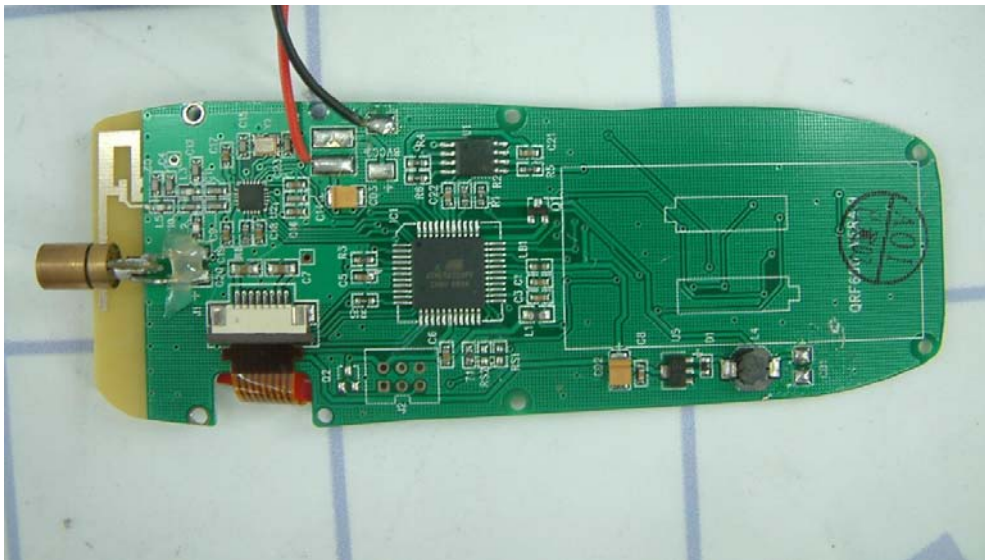
Figure 6 Inside of the EUT
