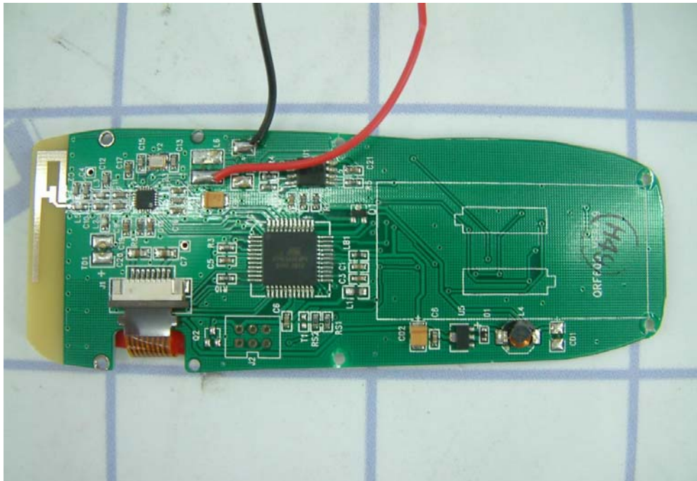
Figure 8 Inside of the EUT
