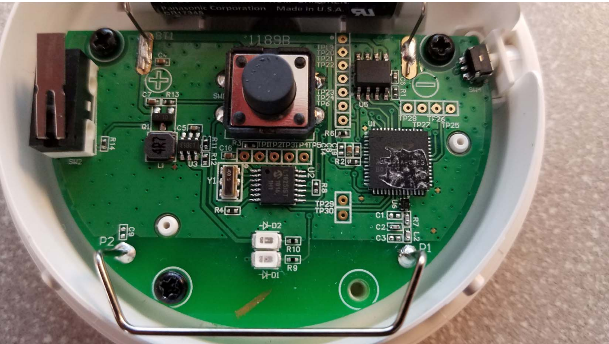
PCB Top with Sticker Removed
