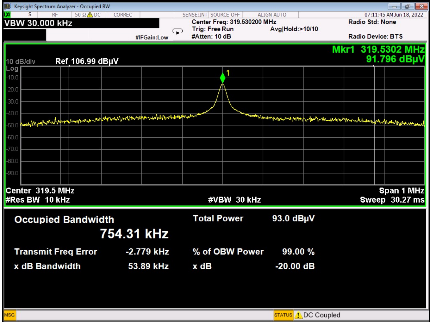
99% Bandwidth Plot
