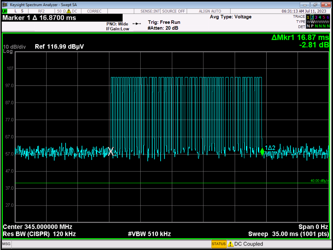
Time of Pulse Train on 35 ms scale
