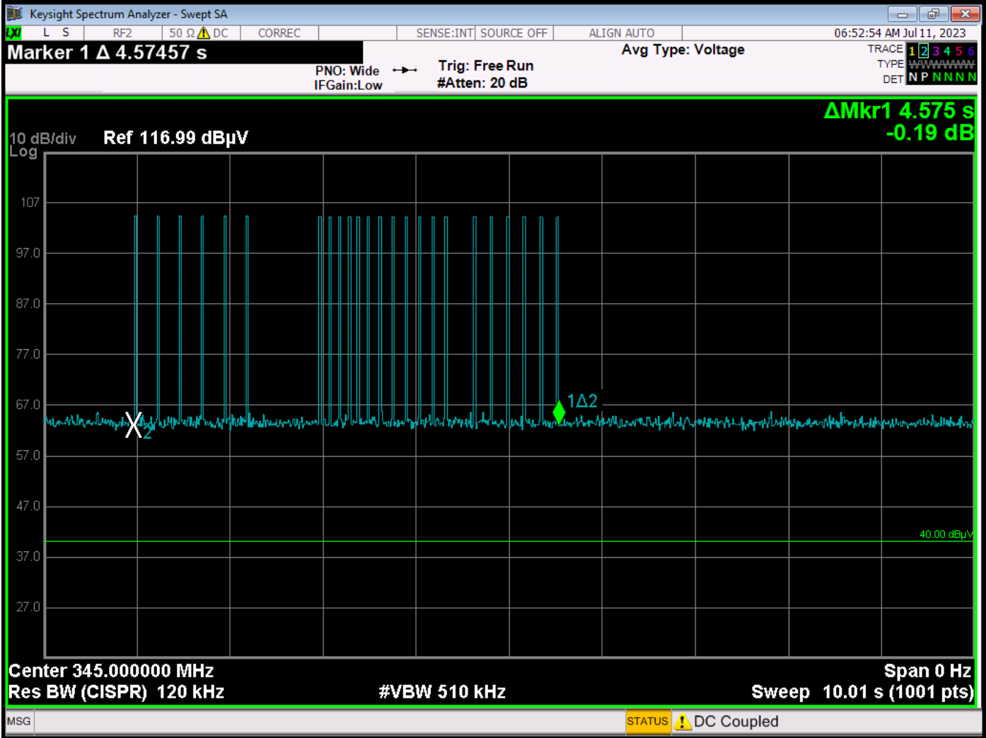
Plot Showing Actual Time of Transmission 4.575 seconds
